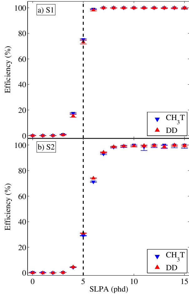
Figure 8: Measured trigger efficiencies as a function of the SLPA. The results from \text{CH}_3\text{T} and DD data sets are compared. a) The S2 filter trigger efficiency for S1 ( \mathcal{E}_{S1}(\text{SLPA}) ). b) The S2 filter trigger efficiency for S2 ( \mathcal{E}_{S2}(\text{SLPA}) ). The vertical dashed lines represent the low filter threshold of 5 phd.
