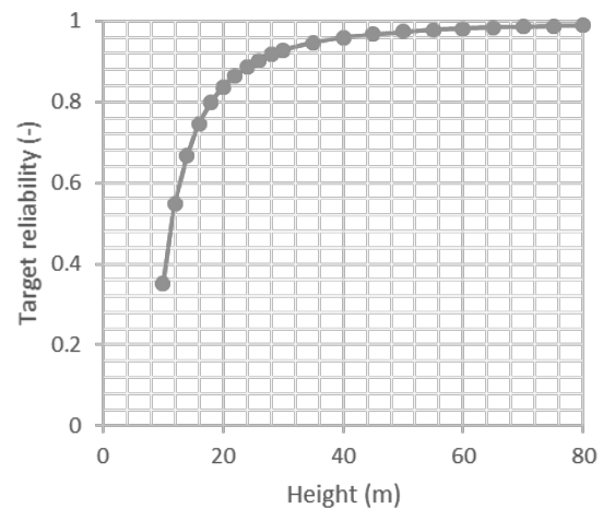
Figure 2 – Relationship between height and target reliability implicit within BS 9999 for an office
