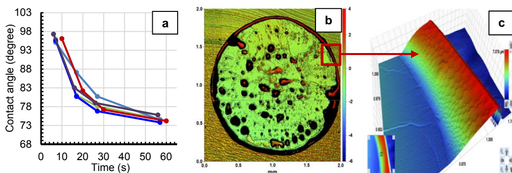
Figure 2: (a) Contact angle \theta of a water droplet on TLC coated glass plate versus time @ T = 25 \text{ }^\circ\text{C} , (b) a top view of the sessile drop (magnification \times 5 ) and (c) a 3D module of the TLCs on the edge of the drop
