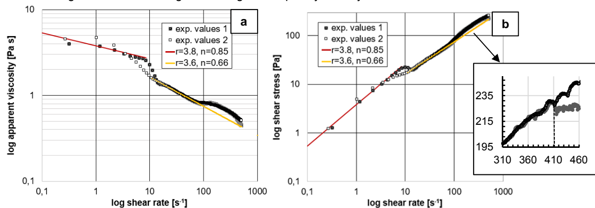
Figure 1: Rheological properties of bulk TLC material. (a) Apparent viscosity vs shear rate ( T=25 \text{ }^{\circ}\text{C} ) compared with Power-law correlations and (b) shear stress vs shear rate ( T=25 \text{ }^{\circ}\text{C} ) with a zoomed view of the TLC behaviour for shear rate values between 300 and 460 \text{s}^{-1} .
