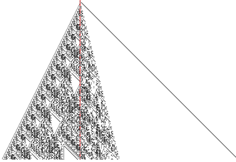
Figure 2: Spacetime diagram of a cellular automaton with memory 20 containing the Rudin–Shapiro sequence.
