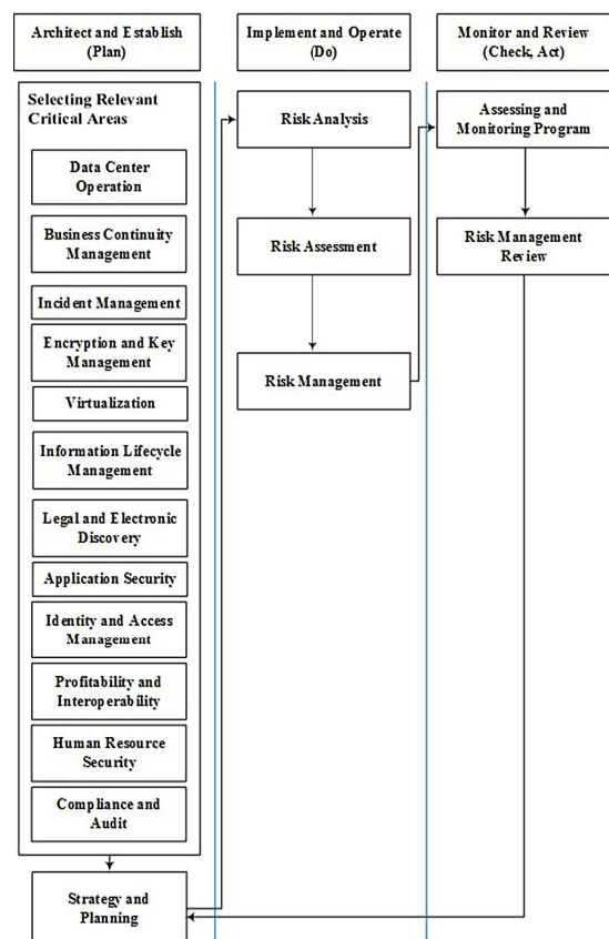
Figure 1. Cloud computing risk management framework proposed by Zhang et al [8]
