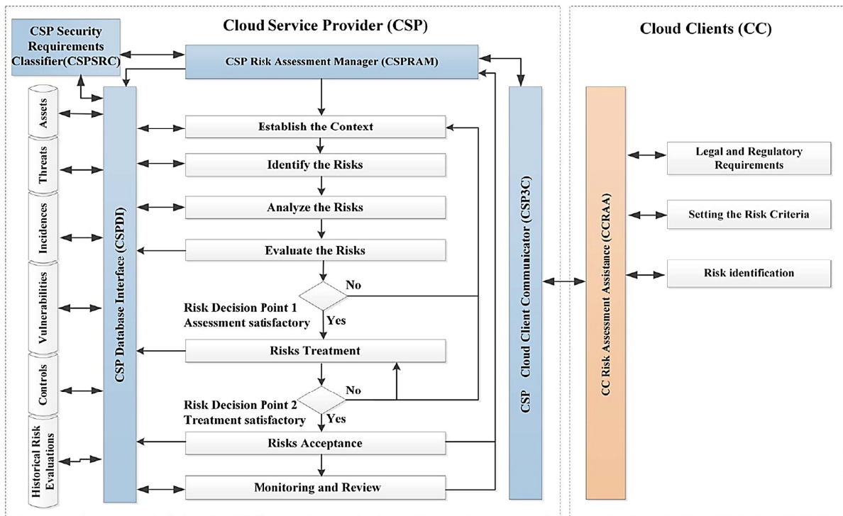
Figure 2. Cloud security risk assessment framework proposed by Albakri et al [7]
