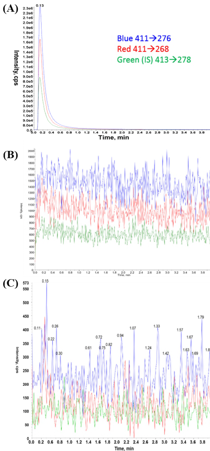
Figure 4: Representative FIA-MS/MS chromatograms of (A) skin tissue extract of 16-7N(G-K)-16 gemini surfactants, (B) double blank skin tissue extract, and (C) double blank PBS extract.
