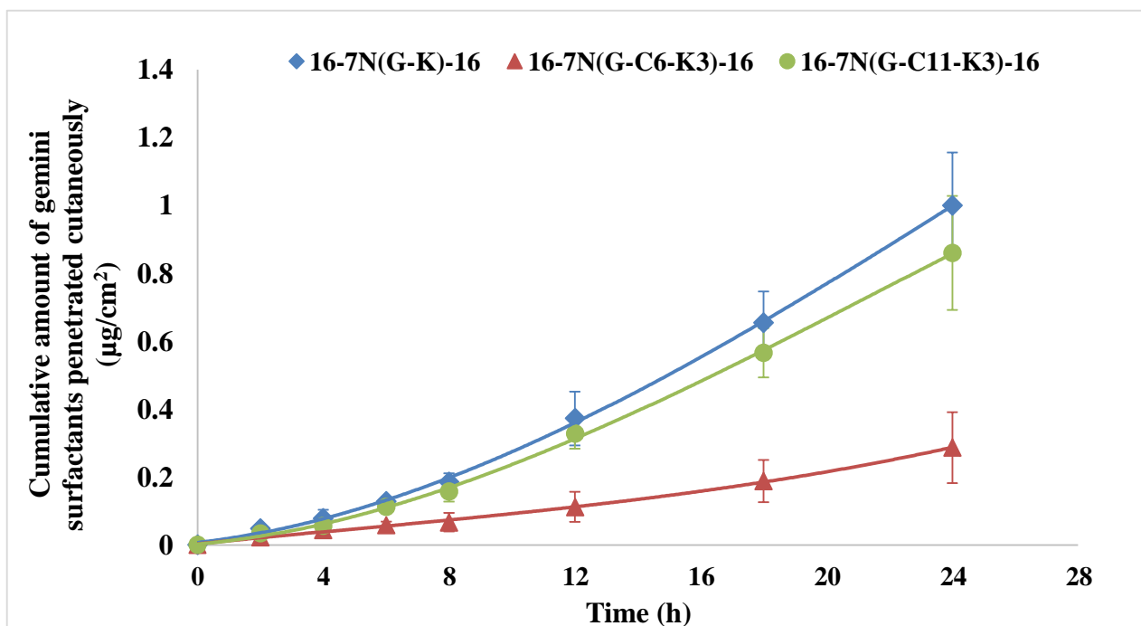
99 Figure 5: Cumulative amount of gemini surfactants ( \mu\text{g}/\text{cm}^2 ) penetrated across the skin into the 100 Franz cell diffusion receptor compartment versus time curves. Results are the average of five 101 measurements, error bars represent standard deviation.
