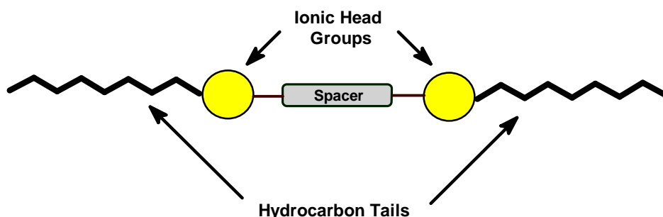
Figure 1: Schematic representation of gemini surfactants showing the two ionic head groups, hydrocarbon tails and the spacer
