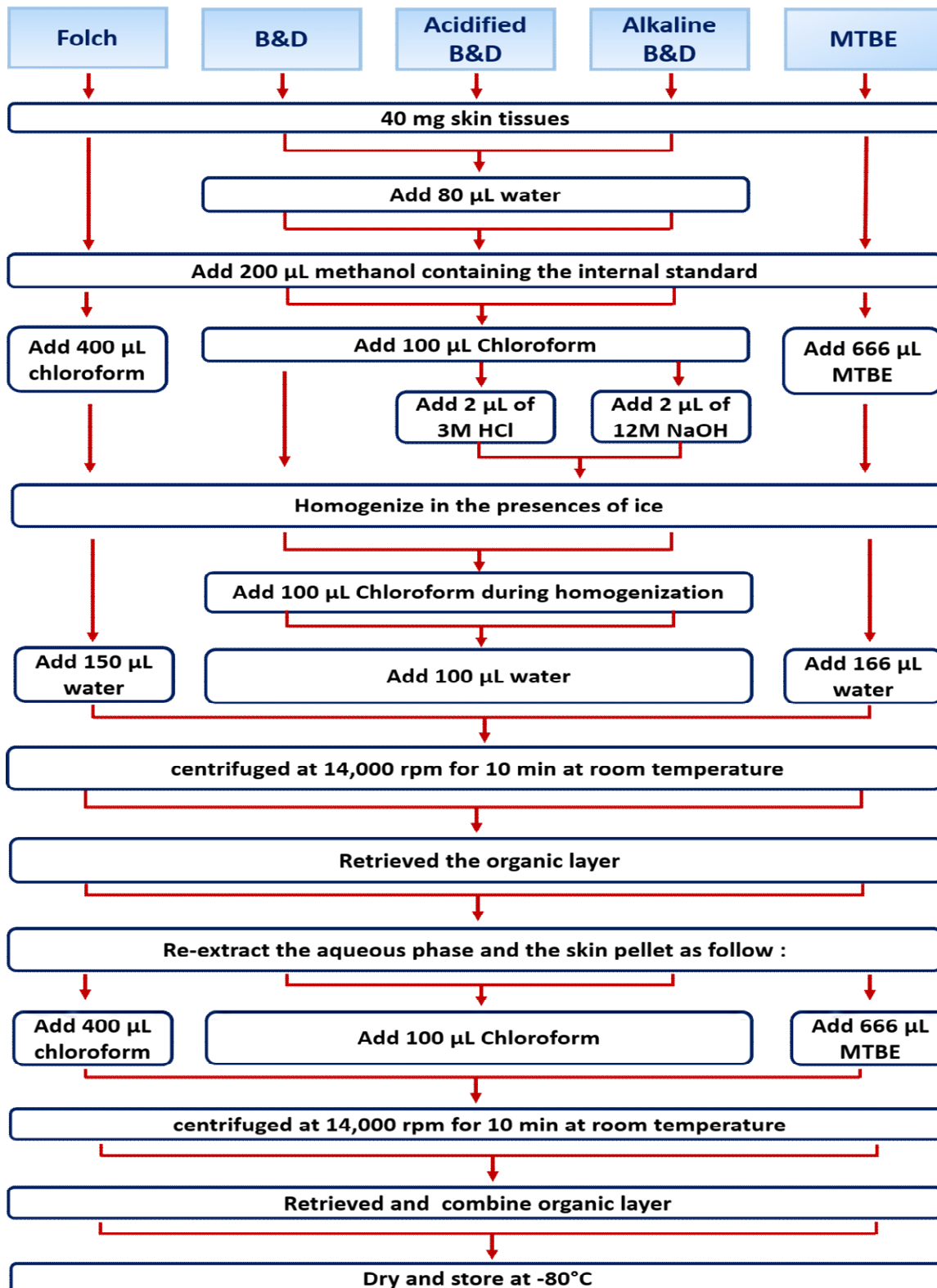
Figure 3: Flowchart summarizing the five evaluated liquid-liquid extraction methods.
