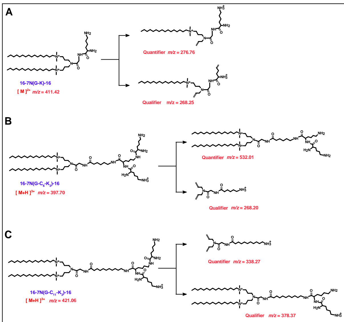
Figure 2: Chemical structure of gemini surfactants 16-7N(G-K)-16 (A), 16-7N(G-C 6 -K 3 )-16 (B) and 16-7N(G-C 11 -K 3 )-16 surfactants showing their precursor ion and the monitored product ions.
