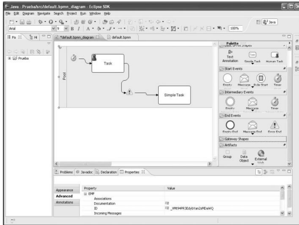
Fig. 4 Editor SBPMN
