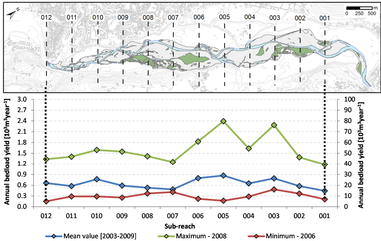
325 Figure S5 – Mean, maximum and minimum modeled annual bedload yield modeled for the 2003–2009 period along the whole study reach
