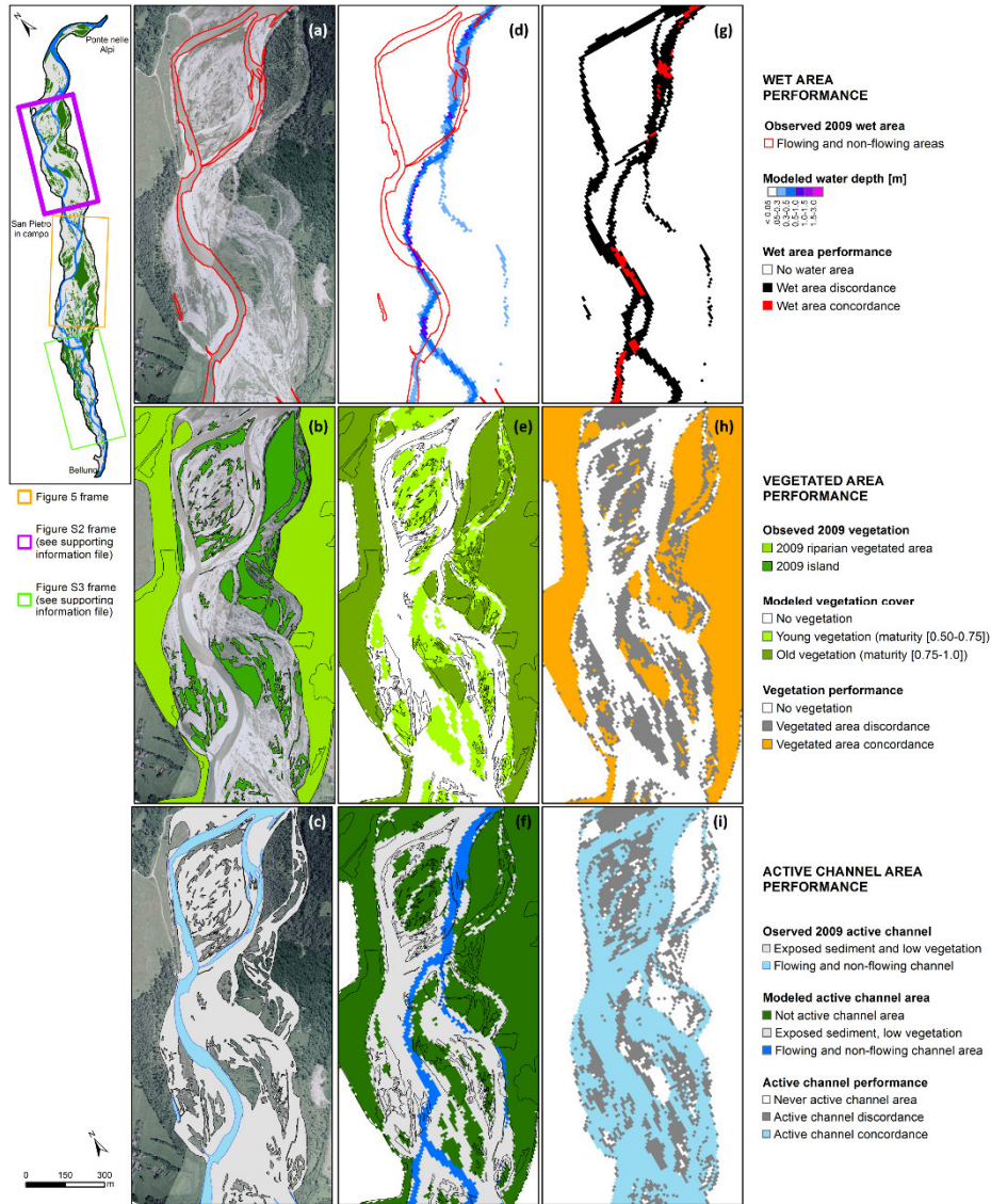
315 Figure S3. Model performance assessment at the end of the calibration runs (upstream frame): (a) wet area (b) vegetated area and (c) active channel digitalized using 5th August 2009 aerial photos; (d) overlay between modeled and observed flowing channel; (e) overlay between modeled and vegetated area; (f) overlay between modeled and observed active channel; (g) wet area performance index calculation; (h) vegetated area performance index calculation; (i) active channel performance index calculation
