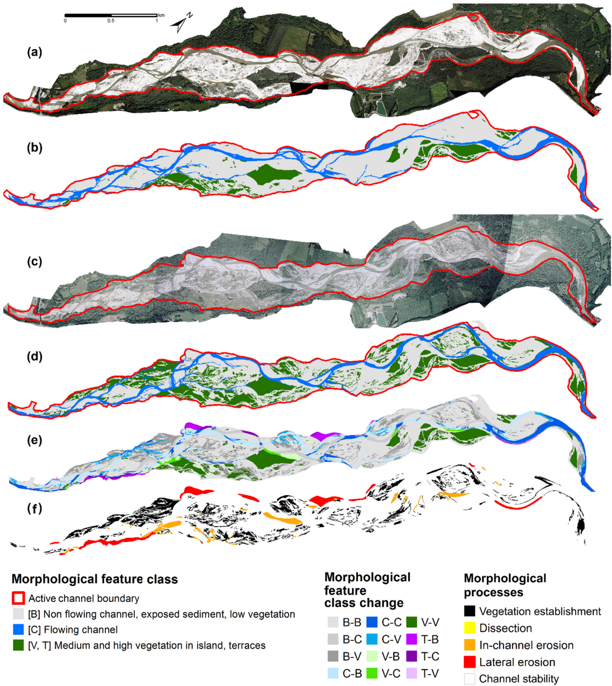
Figure S1 – (a) 2003 aerial photos, (b) 2003 digitized main morphological features, (c) 2009 aerial photos, (d) 2009 digitized main morphological features, (e) morphological features changes in 2003-2009, (f) morphological processes in 2003-2009
