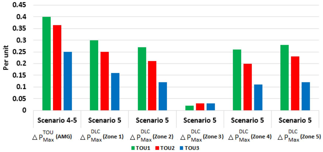
Fig. 8. The DLC parameters for the 4 th and 5 th scenarios.
