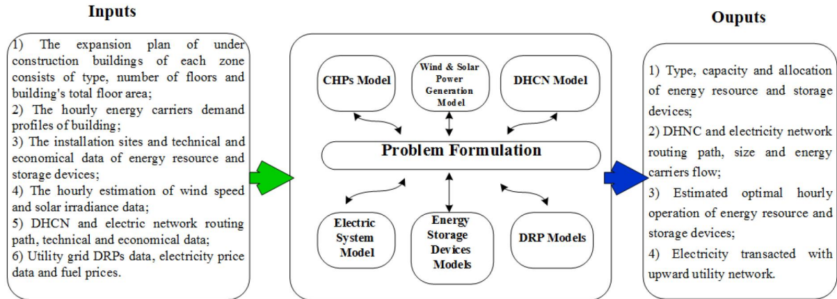
Fig. 2: Schematic diagram of the DERNEP model.
