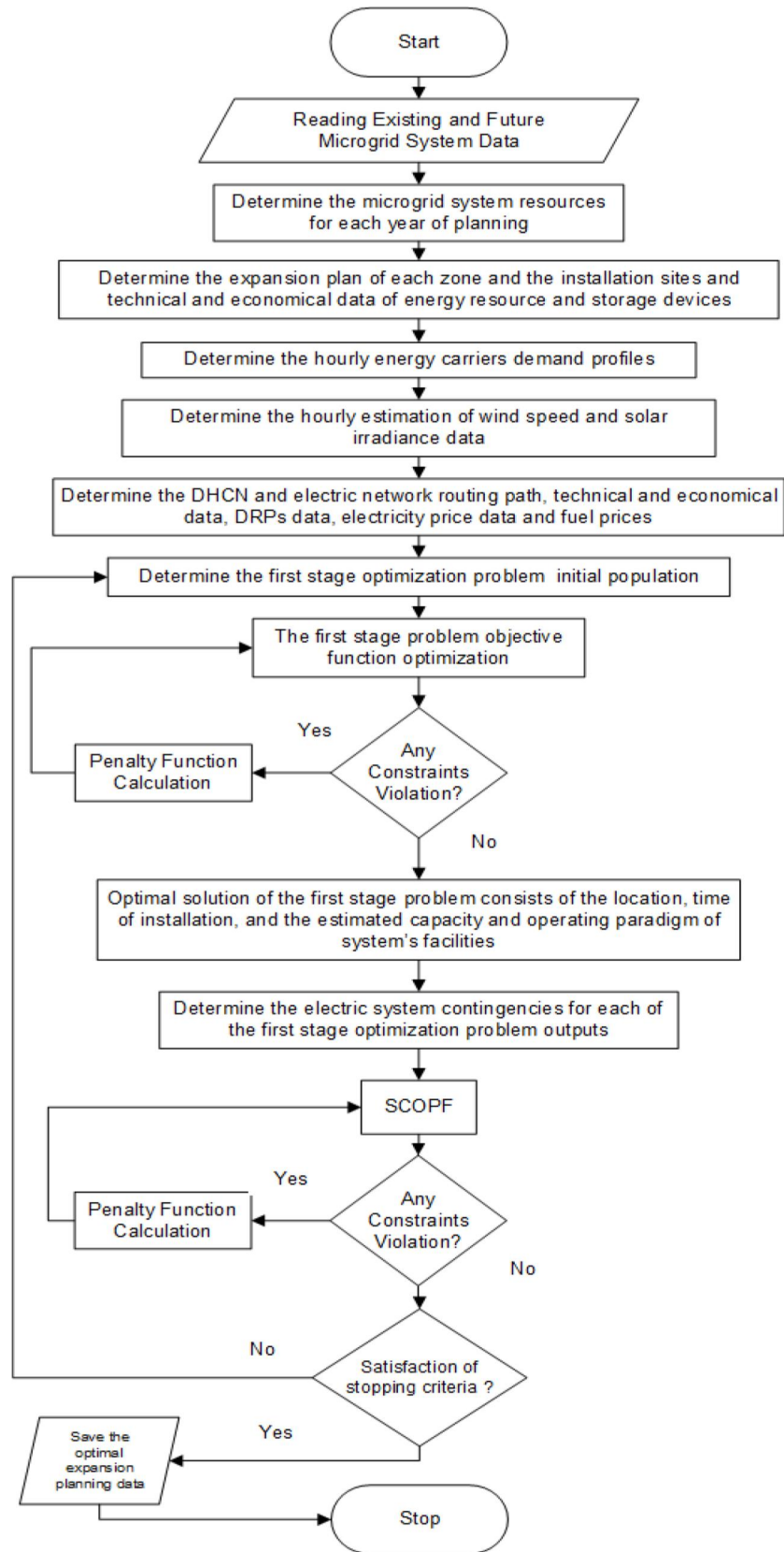
Fig. 3: Flowchart of the DERNEP algorithm.
