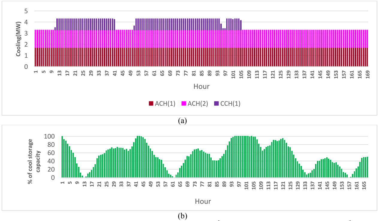
Fig. 17. (a) The stacked column of the estimated values of the 5 th zone optimal cooling dispatch for the 5 th scenario and the first week of June 2023. (b) The 5 th zone optimal cooling storage charge and discharge for the 5 th scenario and the first week of June 2023.
