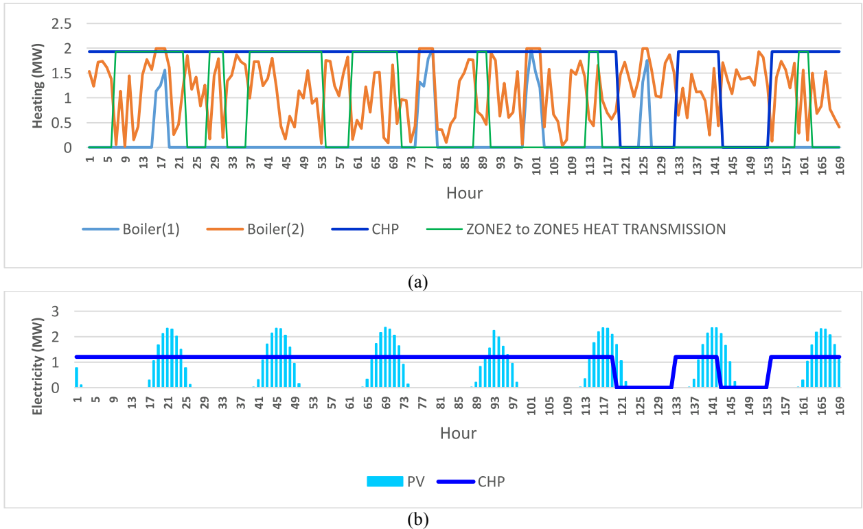
Fig.14. (a) The estimated values of 5 th zone optimal heating dispatch for the 4 th scenario and second week of January 2023. (b) The estimated values of 5 th zone optimal electricity dispatch for the 4 th scenario and second week of January 2023.
