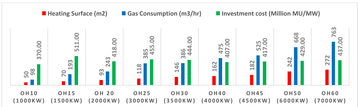
Fig. 6 Boilers data [30].
