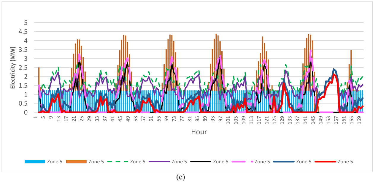
Fig. 21. The estimated electric load, electricity generation, import and export for the 5 th scenario and second week of January 2023 and for: (a) 1 st zone, (b) 2 nd zone, (c) 3 rd zone, (d) 4 th zone, (e) 5 th zone.
