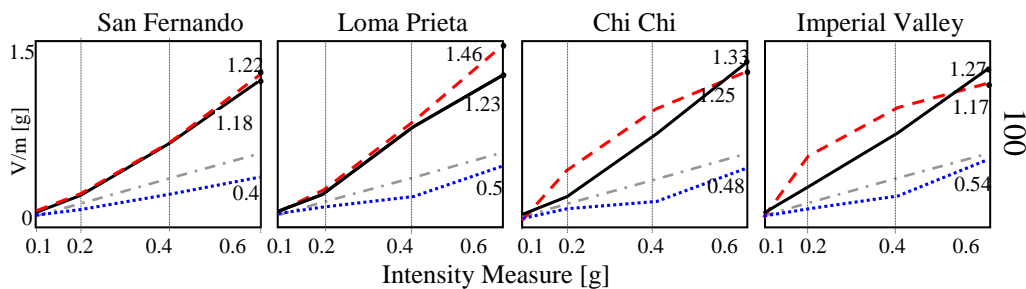
Figure 4. Pseudo-acceleration curves for the various duration scenarios.
