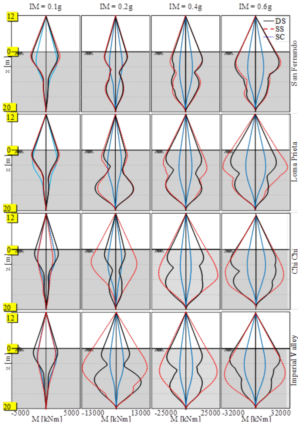
Figure 7. Envelopes of the bending moment for various soil profiles and earthquake events.
