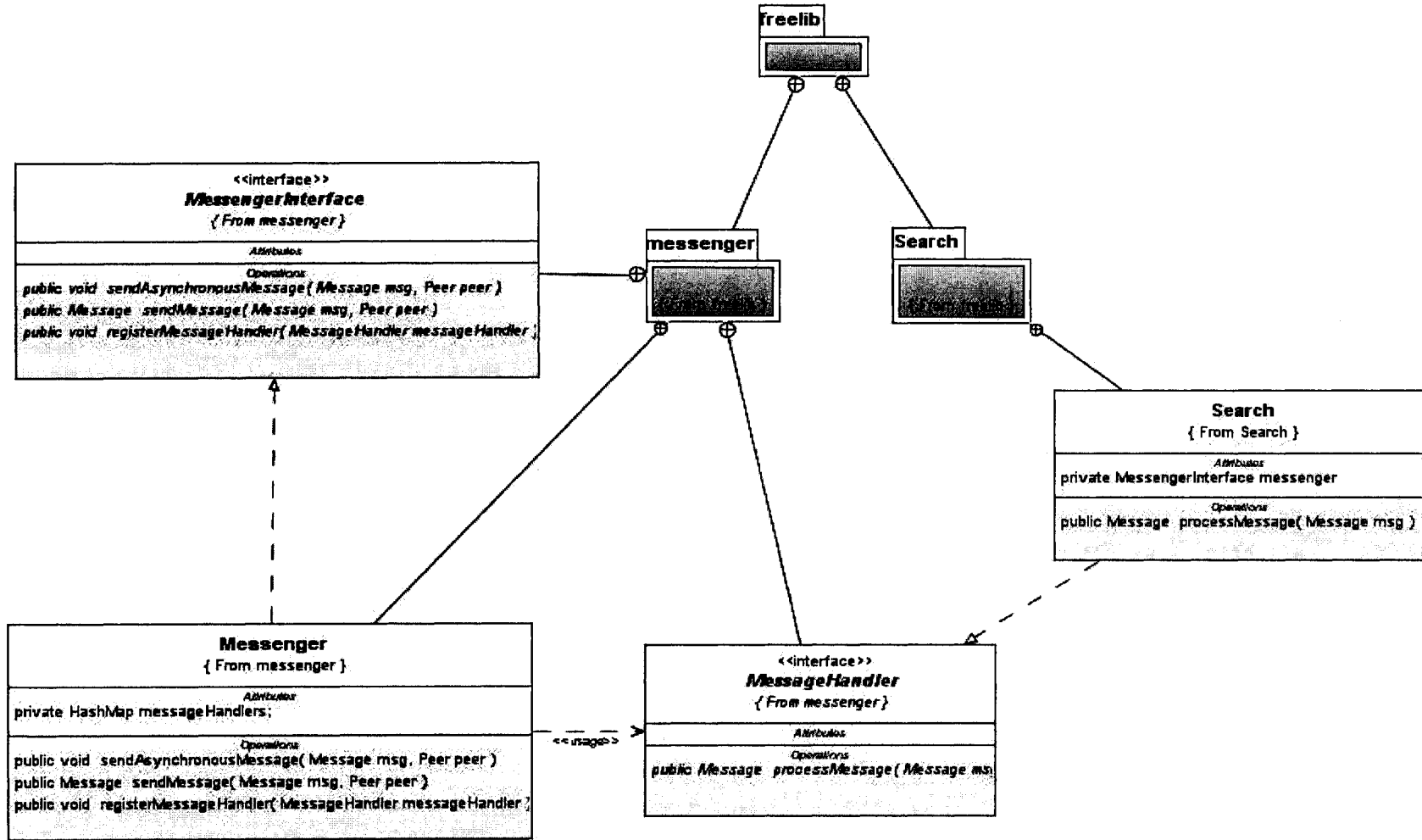
Figure 5.6: Class diagram showing the major classes in the Messenger module and the Search module implementing the MessageHandler interface
