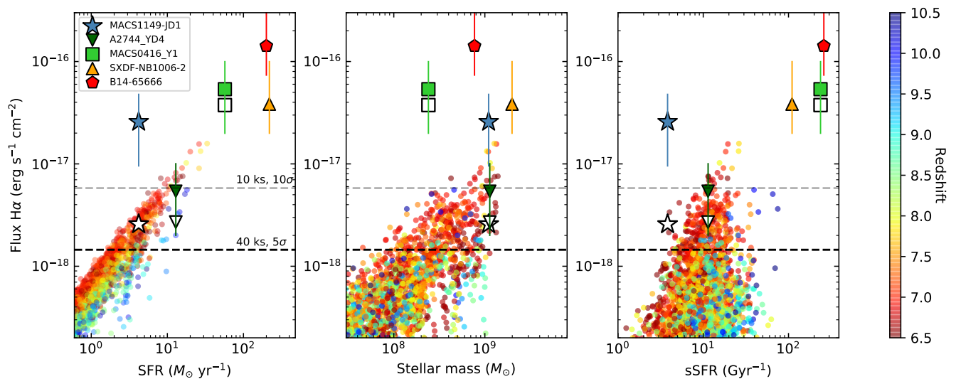
Fig. 2. Predicted H\alpha fluxes as a function of star formation rate (left), stellar mass (middle), and specific star formation rate (right) for the FIRST-LIGHT simulated galaxies at 6.5 < z < 10.5 . Grey and black horizontal dashed lines mark respectively the 10\sigma and 5\sigma limits of medium deep (10 ks) and deep (40 ks) MRS spectroscopic observations. Other known z > 7 galaxies with detected [OIII] 88\mu\text{m} emission lines (Inoue et al. 2016; Laporte et al. 2017; Hashimoto et al. 2019, 2018; Tamura et al. 2019) are also shown with filled symbols (SFR and stellar mass measurements of A2444_YD4 SXFD-NB10006-2 have been corrected for the lower proportion of low-mass stars in the Kroupa IMF relative to the standard Salpeter assumed in Inoue et al. 2016; Laporte et al. 2017, respectively). For these galaxies, ratios of [OIII] 88\mu\text{m} / [OIII] 0.5007\mu\text{m} = 10 and [OIII] 0.5007\mu\text{m} / H\alpha = 1.1 are used to derive the expected H\alpha fluxes (vertical lines show the minimum and maximum expected H\alpha fluxes considering different line ratios of R[OIII] and [OIII] 0.5007\mu\text{m}/H\alpha ; see text for details). For the galaxies magnified by gravitational lensing, such as MACS1149-JD1, A2744_YD4, and MACS0416_Y1, the de-magnified expected fluxes are shown as empty symbols (SFR and M_* measurements refer to intrinsic values).
