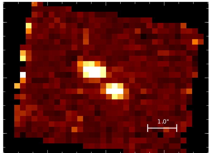
Fig. 4. Simulated B14-65666 system. It illustrates the integrated H\alpha map for a deep (40ks) MRS observations, where two components are simulated as point-like source separated by 1'' , and with metallicities of 0.2 and 0.04 Z_{\odot} .
