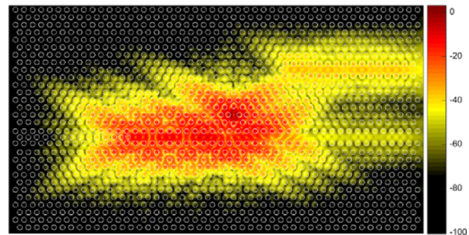
Fig. 5. Example simulation of field distribution ( |E| ) in Fano laser. The color-scale is logarithmic (dB).
