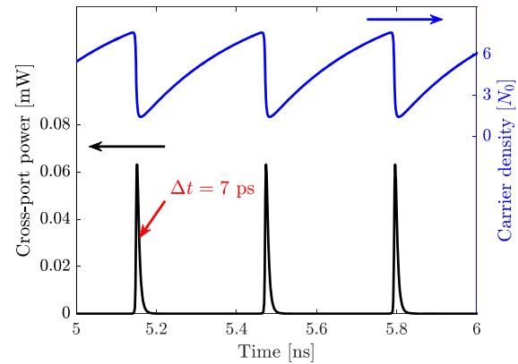
Fig. 10. Cross-port output power and L-cavity carrier density as functions of time in the self-pulsing state, showing typical Q-switching dynamics.
