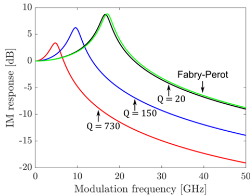
Fig. 11. Intensity modulation response as function of the modulation frequency for a conventional Fabry-Pérot laser (green) and Fano lasers with different values of the nanocavity quality factor (red, blue, black).
