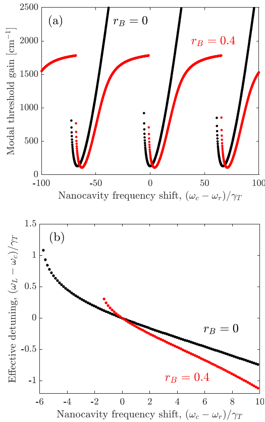
Fig. 7. Variation of (a) laser threshold gain and (b) oscillation frequency when the resonance frequency of the nanocavity is tuned in the absence of a PTE ( r_B=0 , black curves) and in the presence of a PTE ( r_B=0.4 , red curves). The case of zero nanocavity frequency shift corresponds to the laser oscillation frequency being equal to the nanocavity resonance frequency and this reference frequency is denoted \omega_r .
