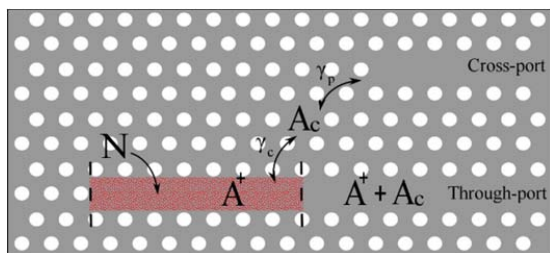
Fig. 4. Schematic of Fano laser implemented in a photonic crystal membrane. The red-hatched area is the laser cavity, where gain is provided by active material. The left mirror is a
