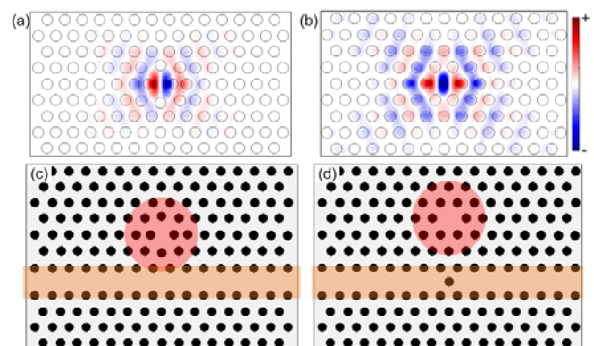
Fig. 2 (a, b) Field pattern (transverse E_y component, colour scale) of the resonant mode of an (a) H0 and (b) H1 photonic crystal point-defect cavity, as calculated using the finite-difference time-domain (FDTD) technique. Black circles are airholes in a semiconductor membrane. Corresponding cavity-waveguide structures are shown in (c) and (d), with (d) showing an example where an airhole in the waveguide below the nanocavity is placed in a partially transmitting element (PTE).
