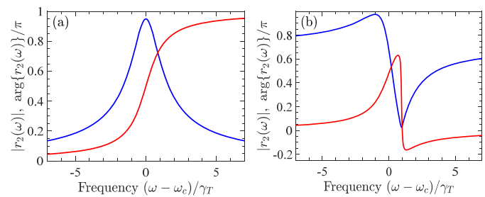
Fig. 3. Calculated reflection amplitude (blue) and reflection phase (red) for a nanocavity side-coupled to a waveguide. (a) Absence of blocking airhole in the waveguide ( r_B = 0 ) and (b) presence of blocking airhole ( r_B = 1/\sqrt{2} ) in the case of coupling to an even mode of the nanocavity. The ratio of the total quality factor of the nanocavity to the coupling Q is Q_T/Q_c = 0.95 in both cases.
