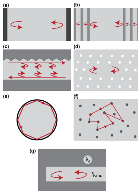
Fig. 1 Different types of laser cavities: (a) Fabry-Pérot laser; (b) Distributed-Bragg-Reflector laser; (c) Distributed-Feedback Laser; (d) Photonic crystal line-defect laser; (e) Whispering-Gallery-Mode laser; (f) Random laser; (g) Fano laser.
