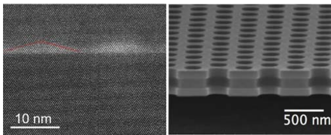
Fig. 14. (a) HAADF STEM microphotograph of a layer of 1.65 ML InAs quantum dots in InP taken in cross-section geometry. The shape of the QD to the left is indicated by red guide lines (b) Example of fabricated membrane structure with embedded active layers, in this case quantum wells.
