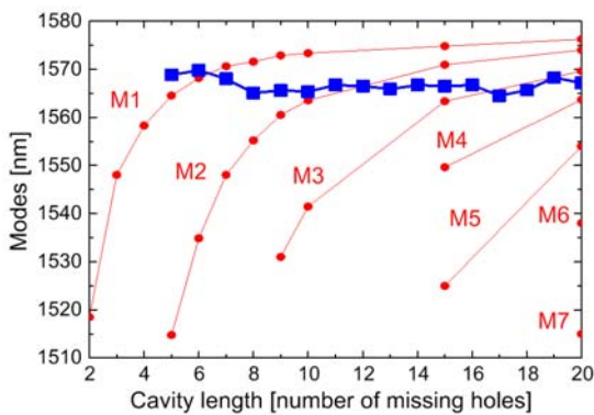
Fig. 17. Measured emission wavelengths versus cavity length for Fano lasers (blue square markers) and ordinary photonic-crystal line-defect cavity lasers (red circular markers). M1–M7 denote the mode order, where M1 is the fundamental mode.
