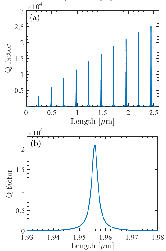
Fig. 6. Variation of quality factor with mirror separation for passive Fano laser cavity. (a) Large-scale variation and (b) zoom-in of variation close to one of the resonances. For these simulations we used Q_T=500 , Q_i=100000 and assumed \alpha=0 .
