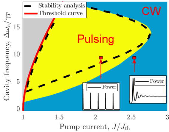
Fig. 9. Phase diagram of laser output as function of pump current and nanocavity frequency, Current is normalised to the minimum threshold current and detuning is normalised to the coupling rate \gamma_T . In the gray region the laser is below threshold (the laser threshold curve is also shown in red), in the blue region the output is continuous-wave, and the region of self-pulsing is shown in yellow. The dashed black line shows the boundary of the self-pulsing regime predicted by a stability analysis. Insets show examples of the temporal variation of the laser intensity in different regions.
