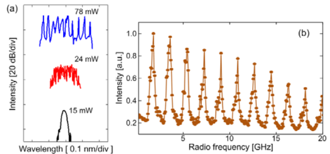
Fig. 18. (a) Measured optical spectra of the Fano laser for pump powers of 15, 24, and 78 mW. For clarity, the spectra are shifted vertically. (b) Measured RF spectrum of the laser power for pump powers of 60 mW.
