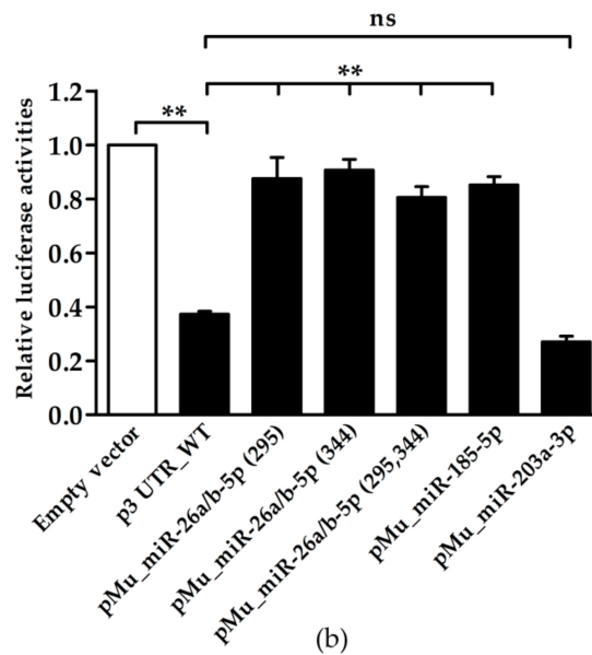
Figure 2. The effect of endogenous miRNAs interacting with the 3'UTR of KIR3DL3 as indicated by luciferase activity. (a) The predicted miRNA binding sites on the 3'UTR of KIR3DL3 are presented in the table. The minimum free energy (mfe) for the binding of each miRNA was calculated by the RNA hybrid program. MiRNA binding sites were mutated by PCR directed mutagenesis and were confirmed by DNA sequencing as shown in the table. The superscript numbers represent the position of the seed sequence binding to the 3'UTR of KIR3DL3. (b) Results from the dual-luciferase assay in YT cell lines when transfected with luciferase constructs of the 3'UTR wild-type (p3UTR_WT) or mutant forms (mutated miRNA-binding site, pMu_miR). The firefly luciferase activity was normalized by renilla luciferase activity and then relative to empty vector. Data are representative of three independent experiments (mean \pm S.E.M.). ** p < 0.01 (Student's t -test).
