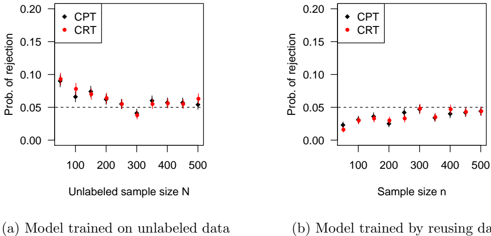
Figure 2: Simulation results for robustness to models trained on unlabeled data or by reusing the data. Details as for Figure 1.
