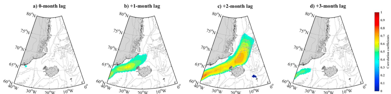
Figure 11. Spatial distribution of the lagged correlation between the monthly depth-mean along-stream velocity at the KGA4 mooring for the NIJ dominant mode, and the monthly wind speed at each grid point in the domain. The lag is listed above each panel. A positive correlation corresponds to the atmospheric signal leading the velocity at KGA4. Only regions with P values \leq 0.05 in the Student's t -distribution test are shown.
