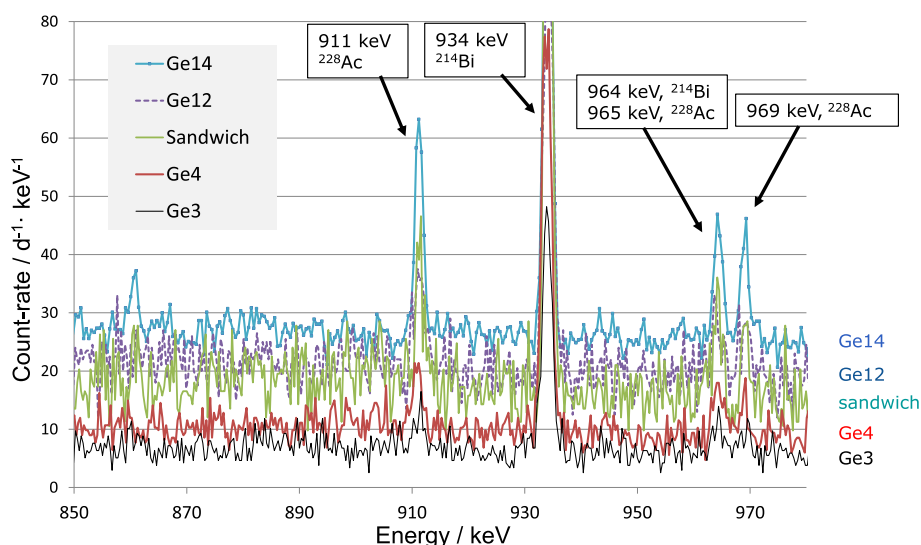
Fig. 5. Like Fig. 4 but for the energy interval 850–980 keV.
