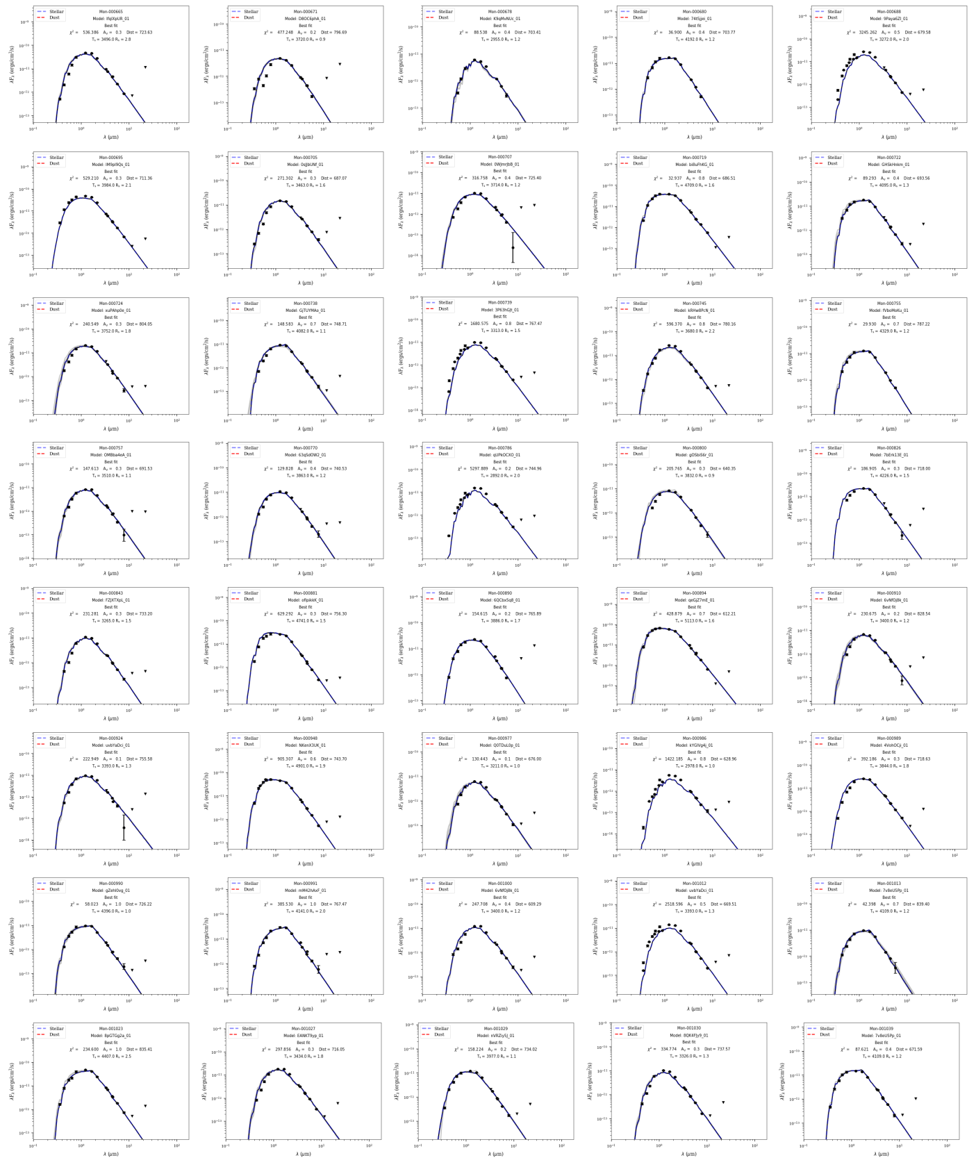
Fig. A.9. The same as Fig. A.7.
