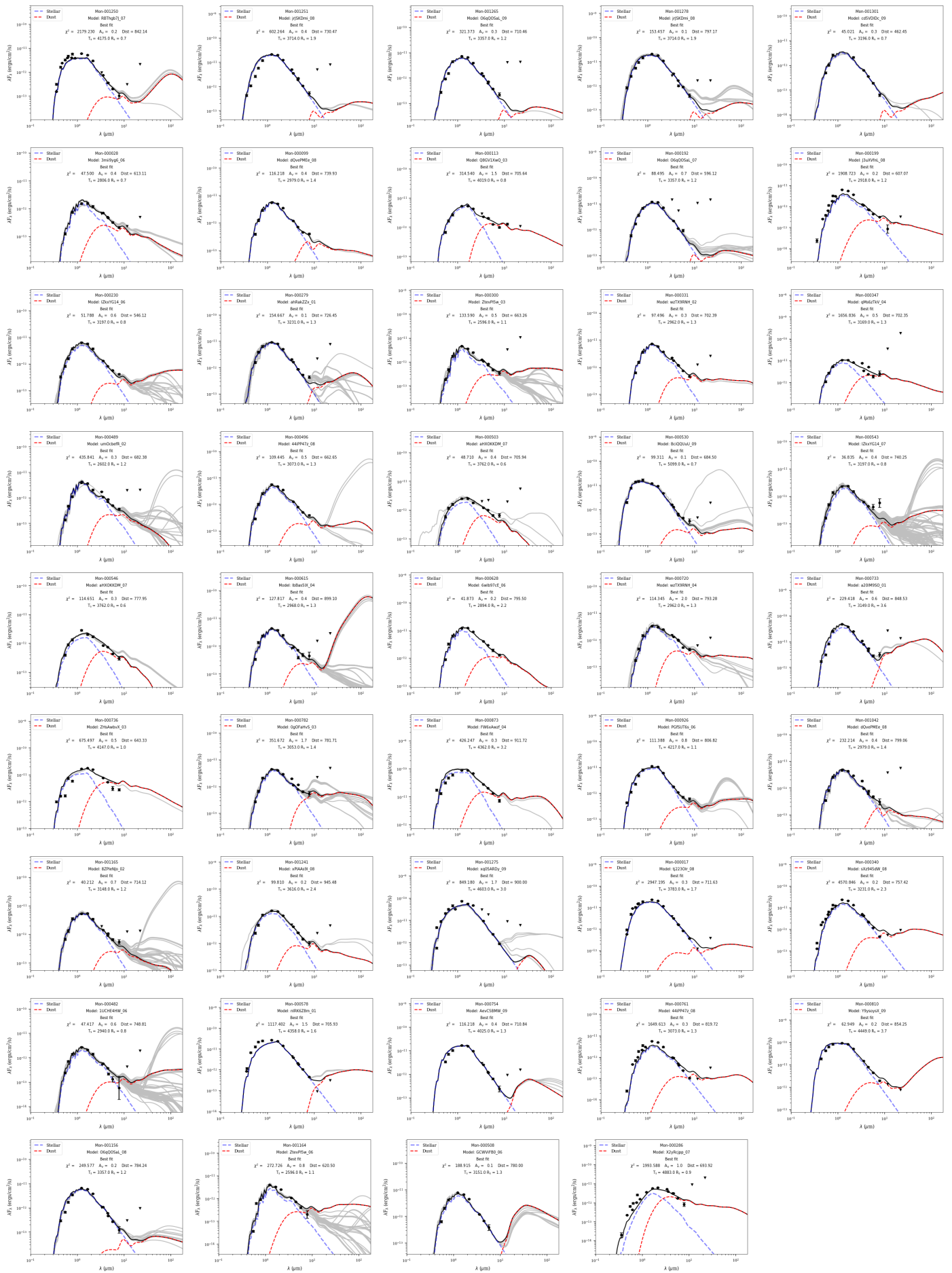
Fig. A.5. The same as Fig. A.4.
