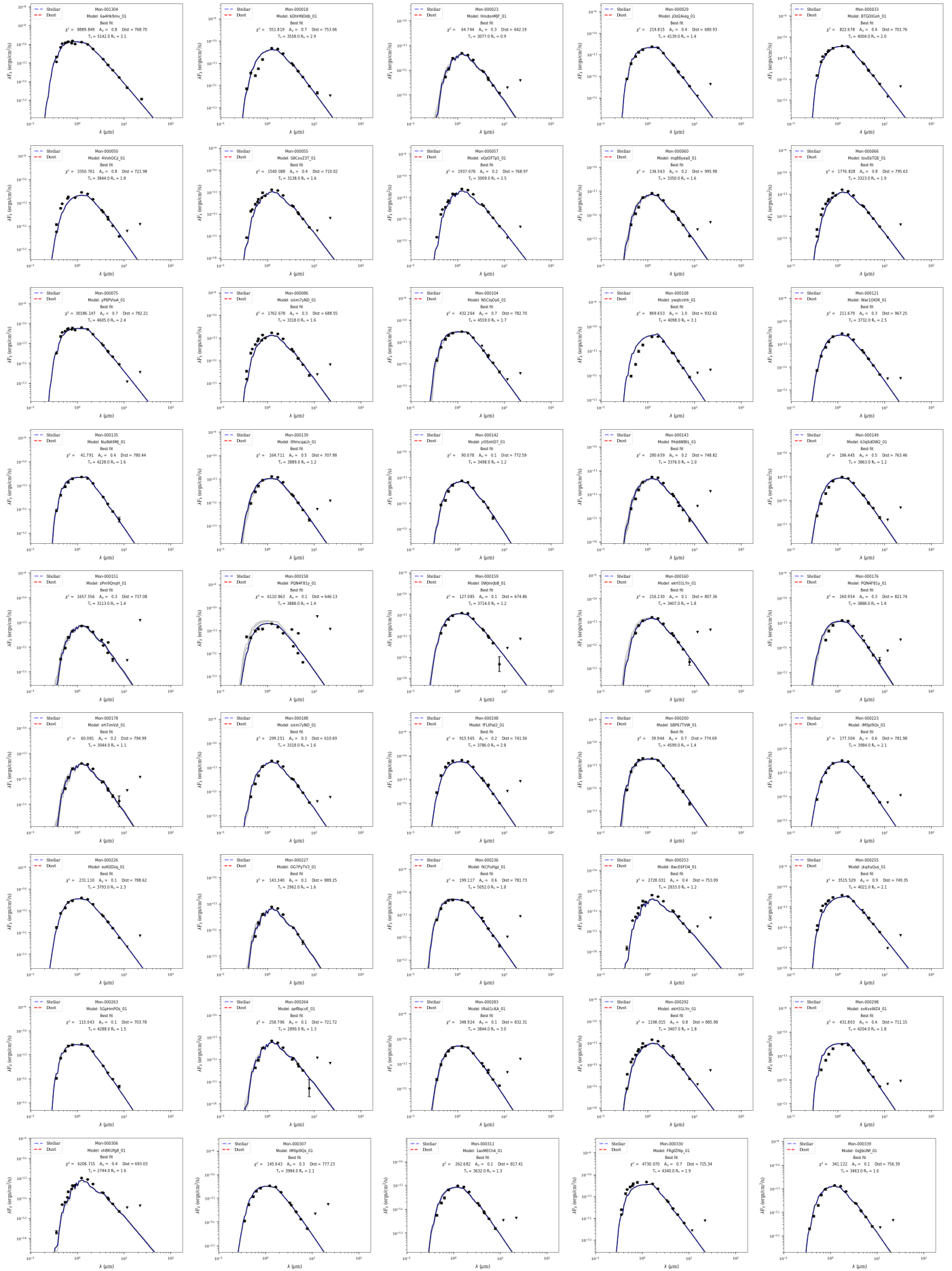
Fig. A.7. The same as Fig. A.1 but for stars classified as diskless.
