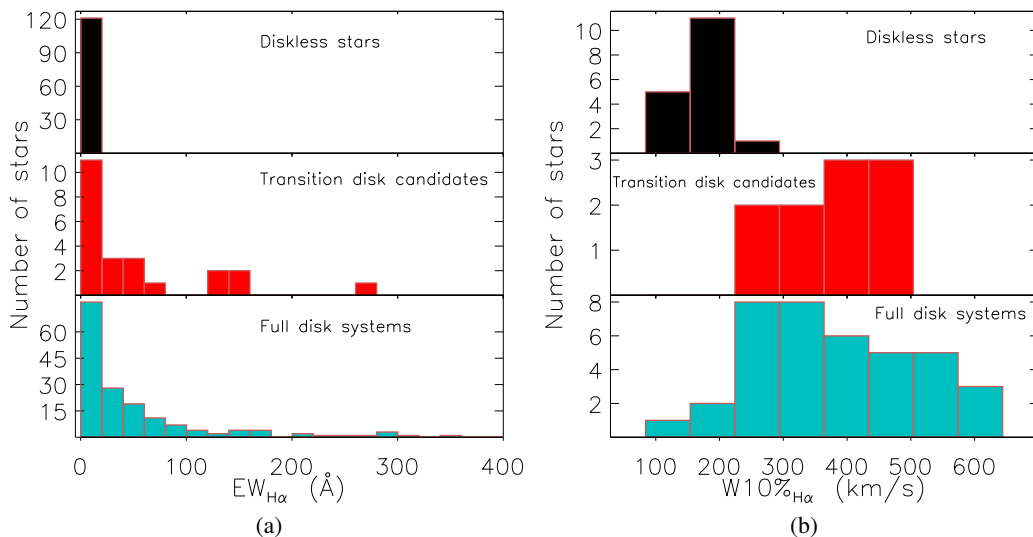
Fig. 8. Distribution of H \alpha emission line parameters. (a) H \alpha equivalent width and (b) H \alpha width at 10% of maximum intensity of our sample of diskless stars (black), transition disk candidates (red) and full disk systems (light blue). Transition disk candidates distributions are more similar to the full disk systems than diskless stars, see the text.
