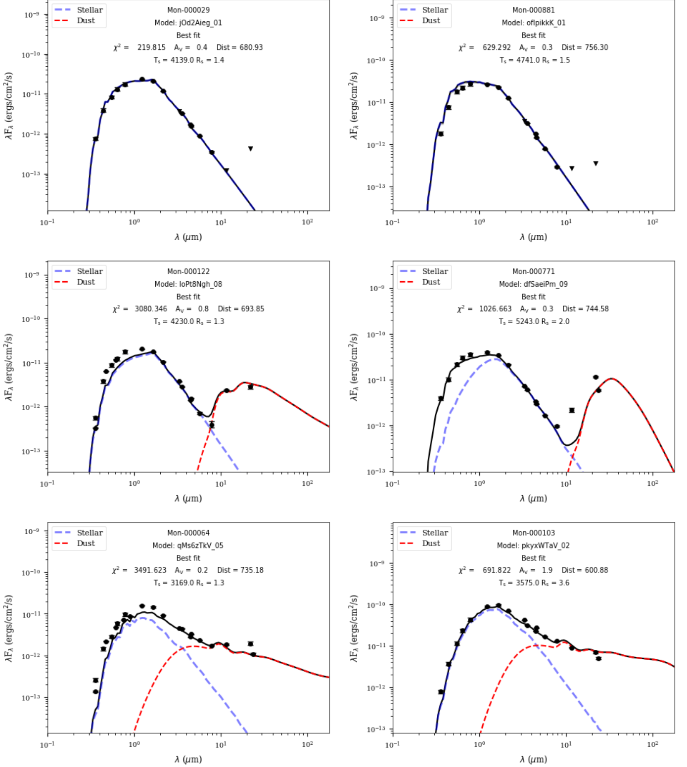
Fig. 2. Examples of synthetic SED fitting, using Hyperion SED code (Robitaille 2017), for our sample of systems classified as diskless stars (top), transition disk candidates (middle) and full disk systems (bottom). The circles show data from the U band ( 0.3\ \mu\text{m} ) to the MIPS 24\ \mu\text{m} band. Triangles, when present, represent the upper limits. The black solid line is the best fit to the SED (Robitaille 2017) and the dashed lines correspond to the stellar (blue) and dust (red) emission components (Robitaille 2011). We found in our sample 7% transition disk candidates, 52% systems with full disks, and 41% diskless stars.
