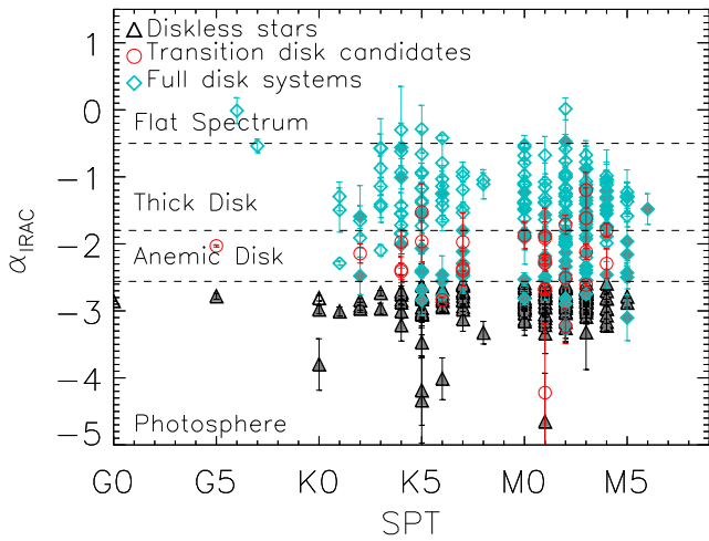
Fig. 6. Slope of the SED from 3.6\mu\text{m} to 8\mu\text{m} ( \alpha_{IRAC} ) measured by Teixeira et al. (2012) as a function of the spectral type obtained by Venuti et al. (2014); Dahm & Simon (2005); Rebull et al. (2002); Walker (1956). Symbols indicate our categorization (notation as in Fig. 4). Our sample of transition disk candidates presents dust in the inner disk similar to anemic disks, which shows that anemic disk systems can be good candidates to transition disks. Systems for which we do not have data at 22/24\mu\text{m} are identified by gray filled symbols.
