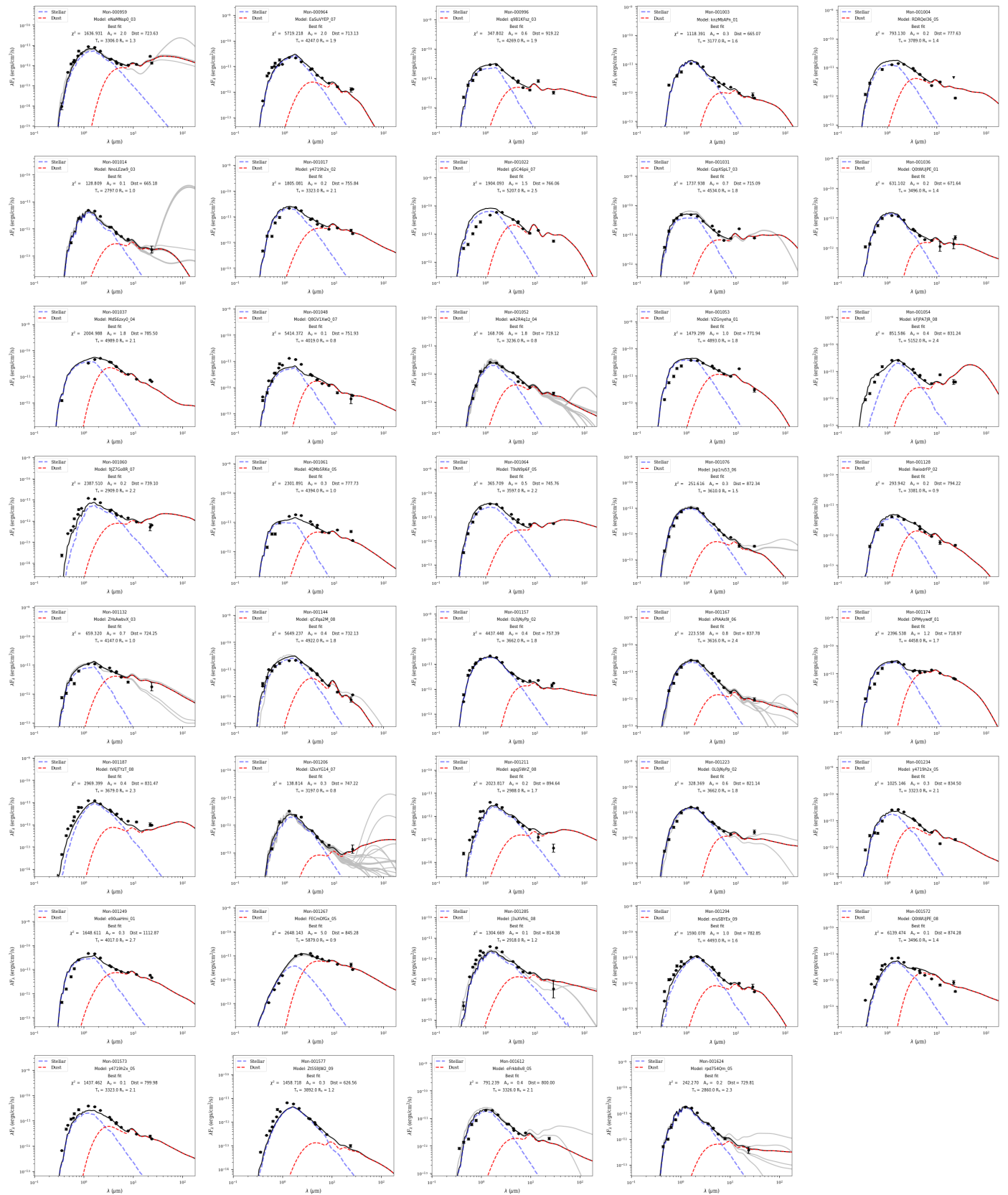
Fig. A.3. The same as Fig. A.1.
