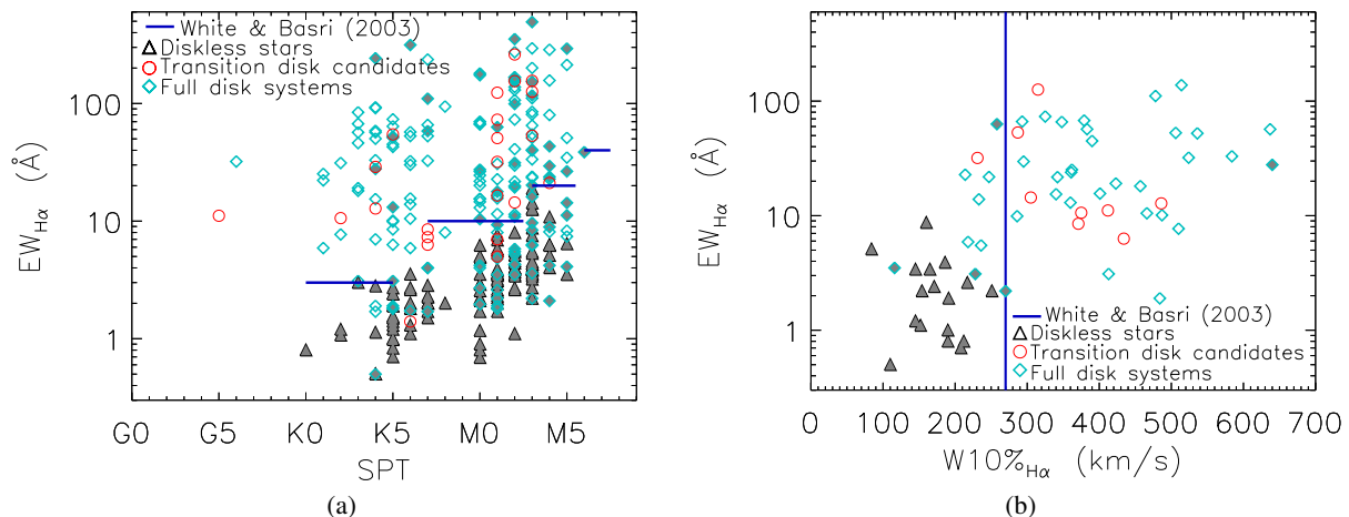
Fig. 7. H \alpha criteria (blue lines) to select CTTS and WTTS (White & Basri 2003). a) H \alpha equivalent width vs. spectral type. b) H \alpha equivalent width vs. H \alpha width at 10% of maximum intensity. Transition disk candidates are predominantly found among accreting systems. Therefore, the presence of a hole in the inner disk does not stop the accretion process, suggesting that gas is flowing through the hole. Systems for which we do not have data at 22/24 \mu m are identified by gray filled symbols.
