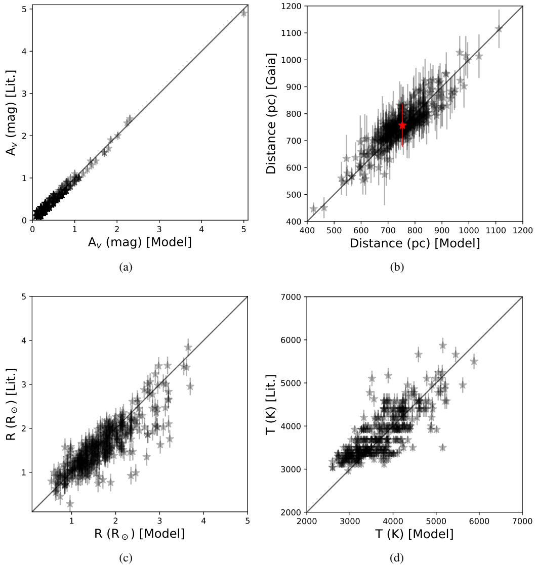
Fig. 1. Stellar parameters modeled with Hyperion SED fitting code (Robitaille 2017) compared to stellar parameters obtained by Venuti et al. (2014). a) A_V , b) distance from the Sun. The red point and error bars represent the mean and standard deviation of the distance of the cluster members studied in this work ( d = 757 \pm 80 pc), c) stellar radii, d) stellar temperatures. A_V and distances are input parameters of the code, while stellar radius and temperature are output parameters of the Hyperion SED Model. The distances were obtained from the Gaia parallax data (Luri et al. 2018). The solid line shows a slope equal to 1. Based on these plots, we conclude that our modeling is doing at least as well as the prior Venuti et al. (2014) modeling.
