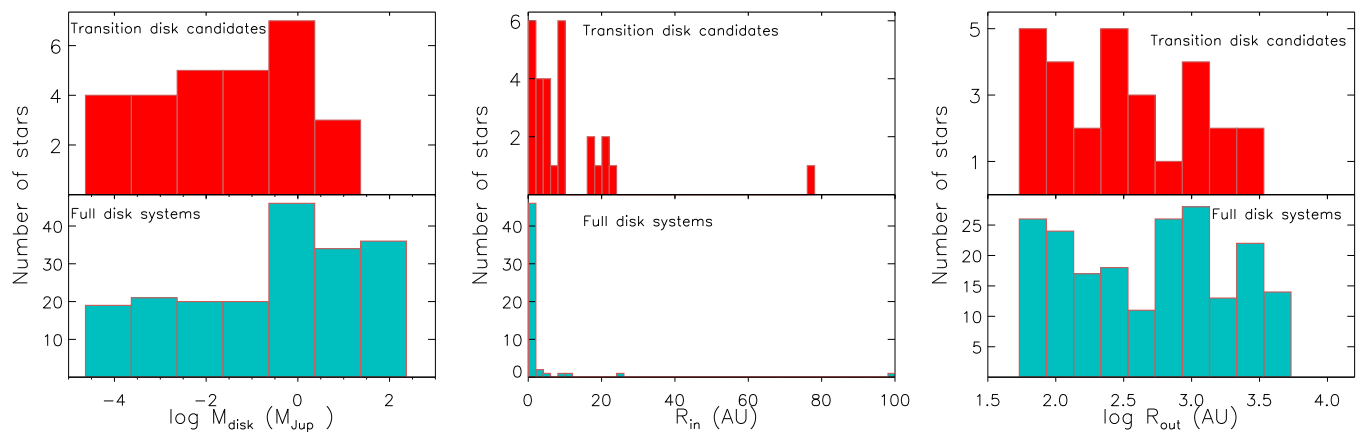
Fig. 13. Distribution of disk parameters obtained by the SED model fitting of transition disk and full disk systems. (Left) Disk dust mass. (Middle) Disk inner radius. (Right) Disk outer radius. For the transition disk sample, the disk inner radius is the inner hole size and for the sample of full disk systems it corresponds to the dust sublimation radius. As the transition disk systems have a disk inner hole, the inner disk radius of the transition disk systems tends to be larger than the full disk systems. The disk mass and the external disk radii are however only estimated values and correspond to lower limits, see text.
