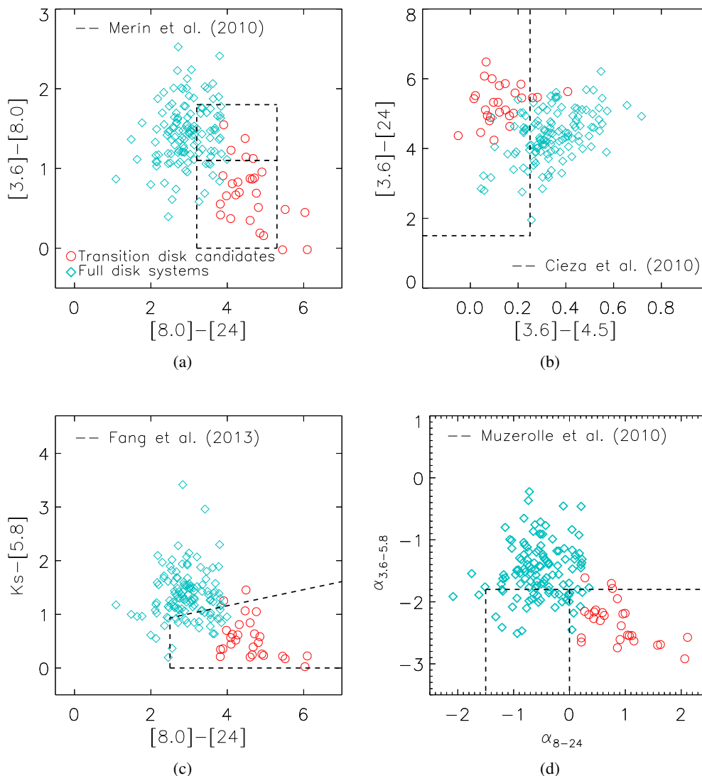
Fig. 5. Different diagrams that are used in previous works to separate transition disk systems from the full disk sample. a) Selection criteria that were used by Merín et al. (2010). Systems that fall in the bottom dashed box are classified as transition disks and systems that fall in the top dashed box are systems with small excess in the IRAC bands. b) Selection criteria used by Cieza et al. (2010). The dashed lines separate the transition disks. c) Selection criteria from Fang et al. (2013). Systems that fall in the dashed region are transition disks. d) Selection criteria from Muzerolle et al. (2010). Systems in the left dashed box are classified as weak-excess sources and systems that lie in the right dashed box are transition disks. Almost all of our transition disk candidates fulfill the selection criteria from the literature.
