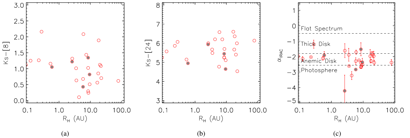
Fig. 15. Disk diagnostics as a function of disk hole size for our sample of transition disk candidates. (a) Near-IR color, (b) mid-IR color, and (c) \alpha_{IRAC} index. Gray filled symbols identify systems that fall in the region where the inner disk hole can be explained by X-ray photoevaporation.
