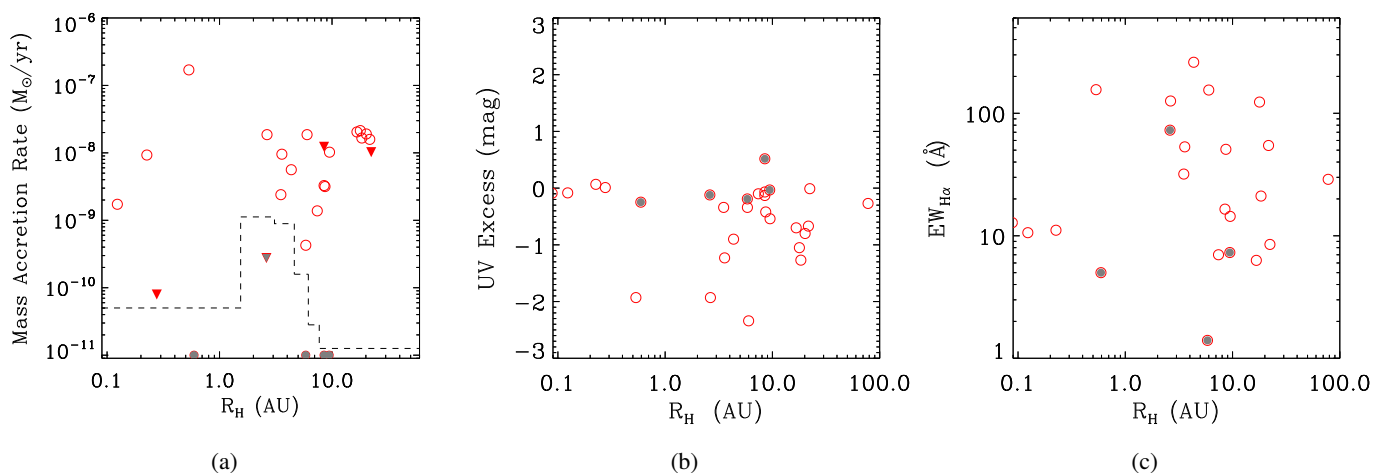
Fig. 14. Accretion diagnostic as a function of disk hole size for transition disk candidates. (a) Mass accretion rates are from UV excess (preferentially) (Venuti et al. 2014) and from H\alpha equivalent width (Sousa et al. 2016). For WTTS, we fix the value of the mass accretion rate at 1 \times 10^{-11} M_{\odot} \text{yr}^{-1} . The upside down triangles correspond to the upper limits of the mass accretion rate. The dashed line represents the region where the inner hole can be explained by X-ray photoevaporation (Owen et al. 2011, 2017). Only \sim 18\% of our sample of transition disk candidates can be explained by X-ray photoevaporation of the inner disk by stellar radiation. (b) UV emission excess (Venuti et al. 2014). (c) H\alpha equivalent width (Sousa et al. 2016; Dahm & Simon 2005). Gray filled symbols identify systems that fall in the region where the inner disk hole can be explained by X-ray photoevaporation.
