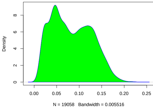
Figure 4: Threshold (T) estimation: Kernel density function obtained for the training data.
