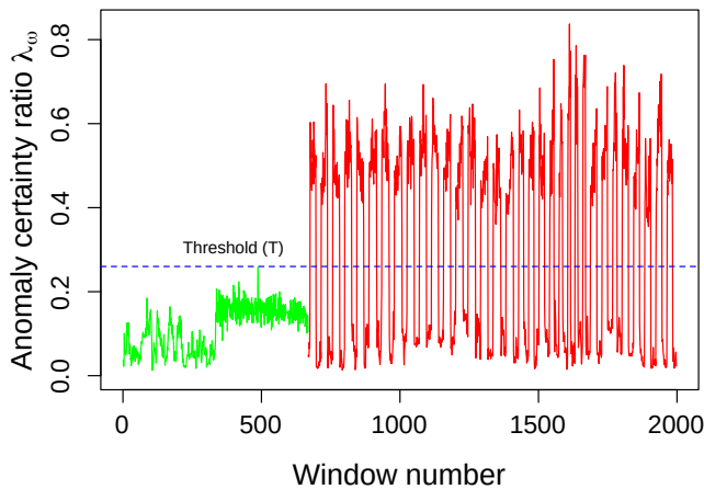
Figure 7: Monitoring for Gear gauge message spoofing attack: Green line denotes \lambda_\omega values during the benign data. Red line denotes \lambda_\omega values during the attack data. Blue dotted line denotes the threshold T at \lambda_\omega = 0.26 .
