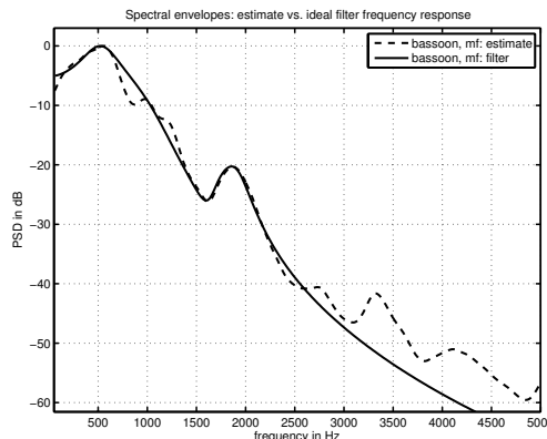
Figure 2: Modelled filter frequency response (solid) and spectral envelope estimate (dashed) for bassoon.
