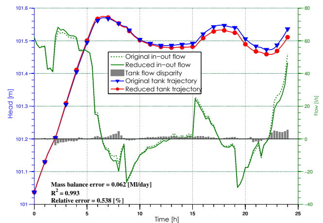
Figure 3. Typical discrepancy in tank level in the original and simplified models.
