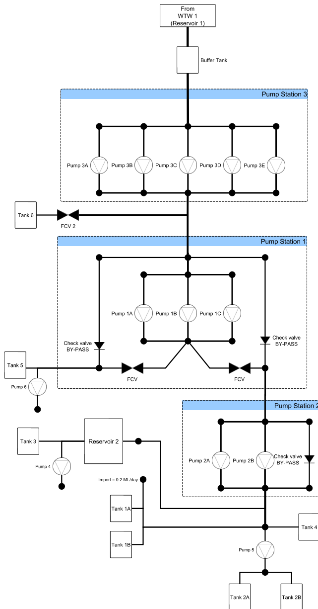
Figure 2. A schematic of the network.
