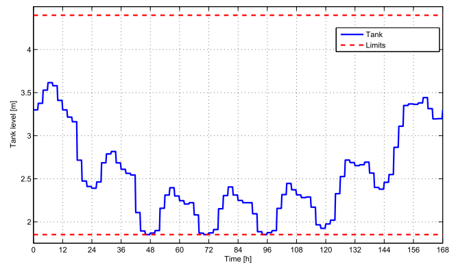
Figure 6. An example tank level trajectory.
