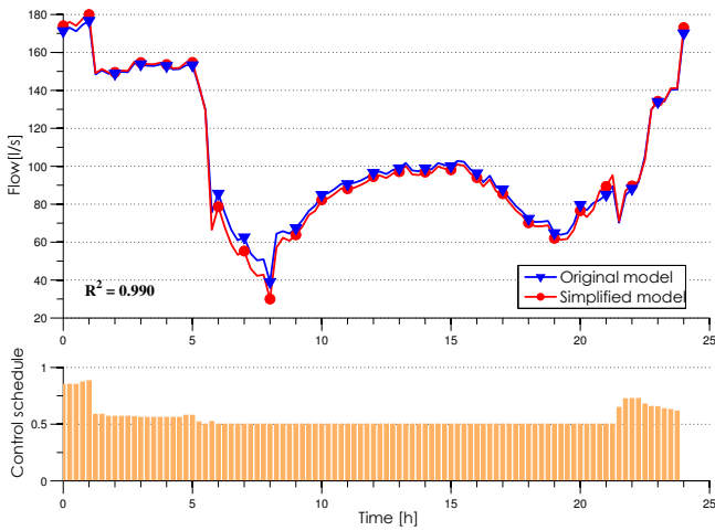
Figure 4. Typical discrepancy in performance of a pump station in the original and simplified models.
