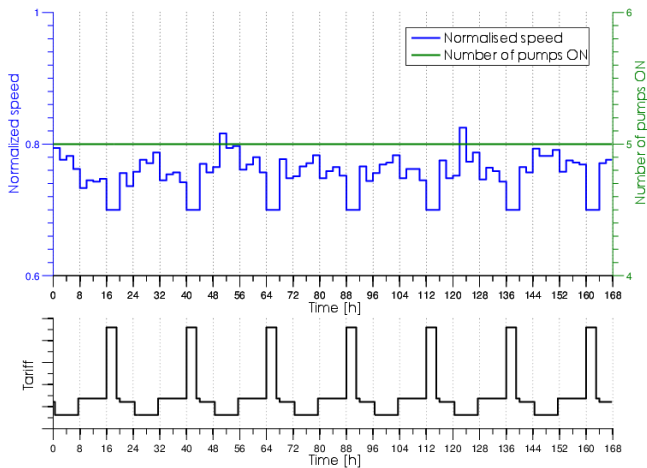
Figure 5. An example schedule for the largest pump station.
