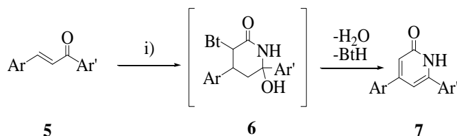
Scheme 1. Reagents and conditions: i) BtCH 2 CONH 2 , NaOH, EtOH, reflux.
