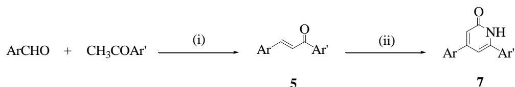
Scheme 2. Reagents and conditions: (i) NaOH(aq), MeOH, rt, 51-94% yield. (ii) CH 3 CONHCH 2 CONH 2 , Cs 2 CO 3 , DMF, 150°C, 1h, 6-60% yield.
