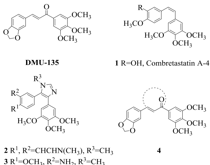
Figure 1. Incorporation of a heterocyclic ring into chalcone and stilbene structures.
