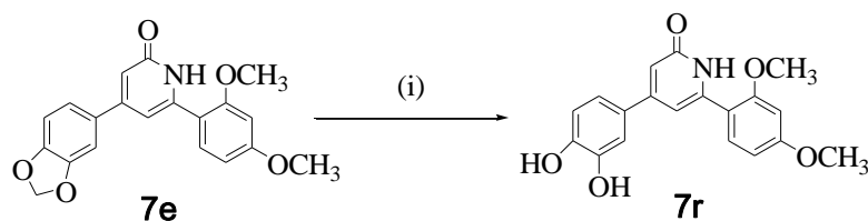
Scheme 3. Reagents and conditions: (i) \text{BCl}_3 , \text{CH}_2\text{Cl}_2 , -5^\circ\text{C} , 1h, 59%.
