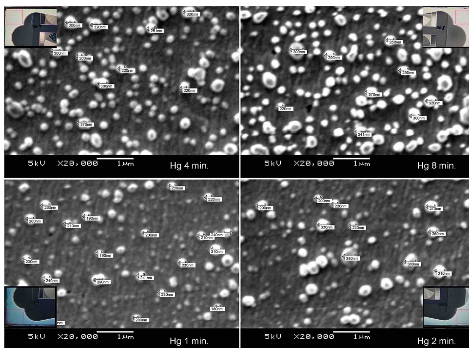
Figure 87. DagTest 3-18-2011. Solarized highlight particle size and frequency.
