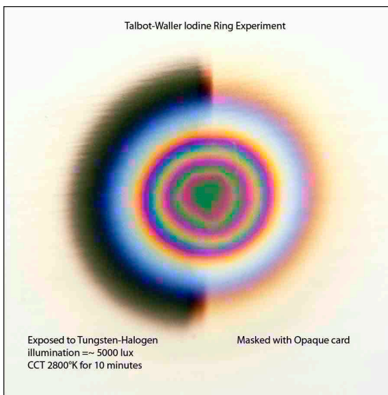
Figure 33. DagTest 9-19-2011, Iodine Ring Experiment.
