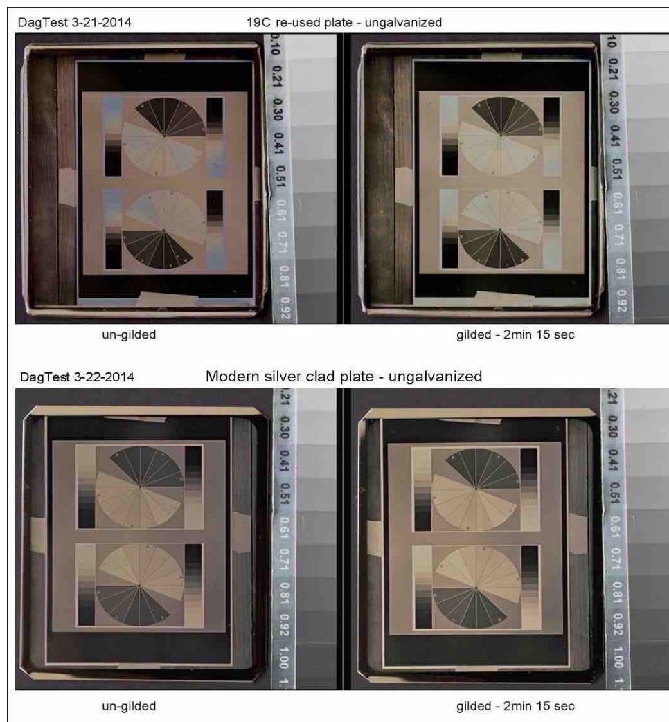
Figure 93. DagTest 3-21-2014. Nineteenth century plate (top). DagTest 3-22-2014. Modern plate (bottom). Before and after gilding.
