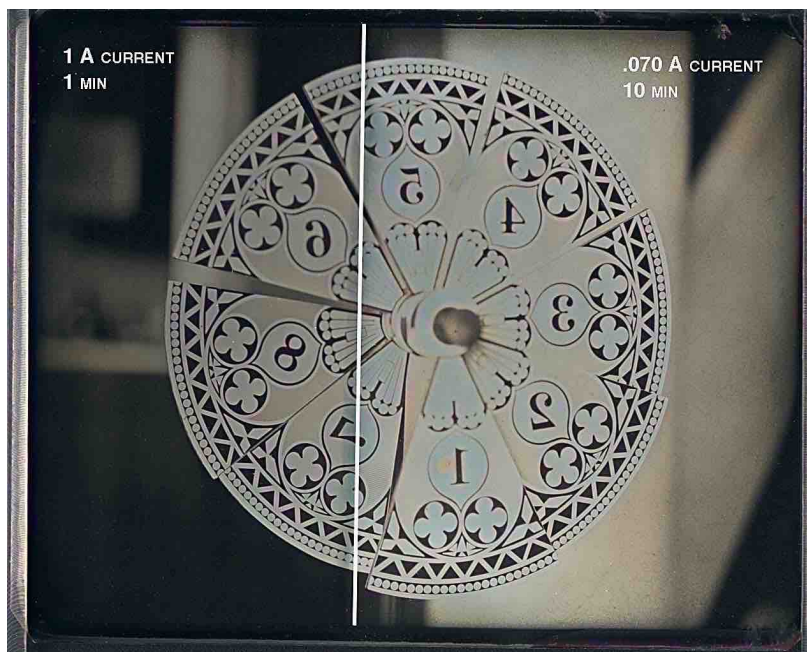
Figure 27. Plating current test, 2005. The photosensitivity difference between a hard, fine-grained silver deposit produced with high current density (left), and a soft large-grained silver deposit produced with low current density (right).
