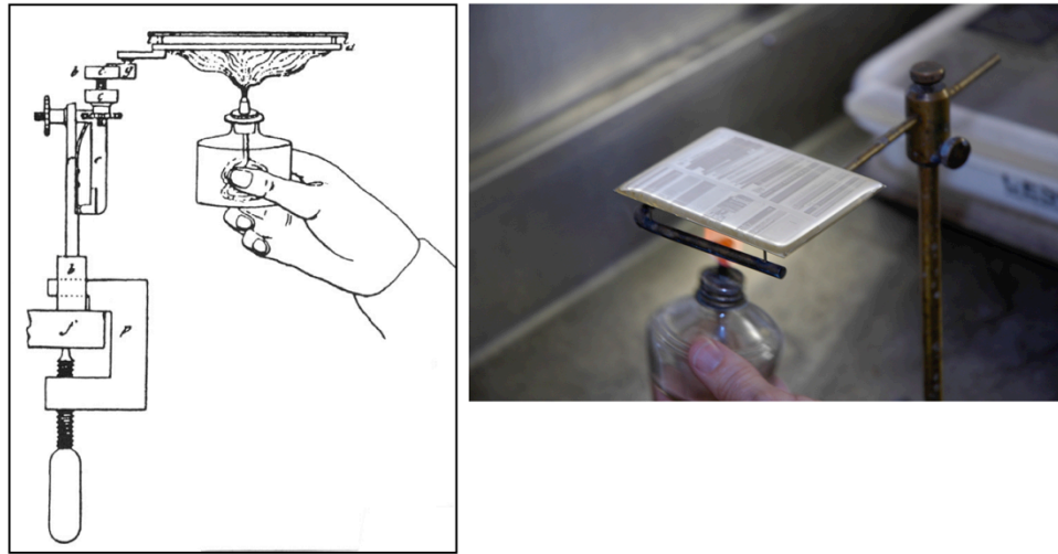
Figure 10. Gilding illustration adapted from E. de Valicourt (left). Gold toning a quarter-plate (right).
