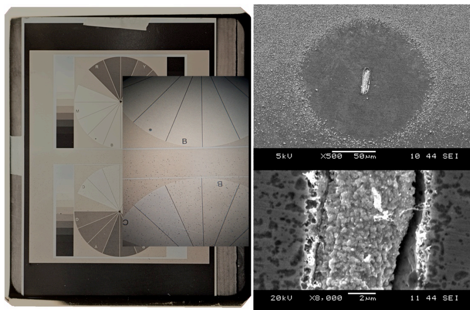
Figure 28. Dag Test 3-23-2014. The inset image from a light microscope shows dozens of black spots on the un-galvanized side that did not form on the galvanized side. SEM image of a black spot magnified 500X shows the insensitive circular void (upper right). SEM image showing silver grain cluster polishing residues trapped in a surface defect (lower right).
