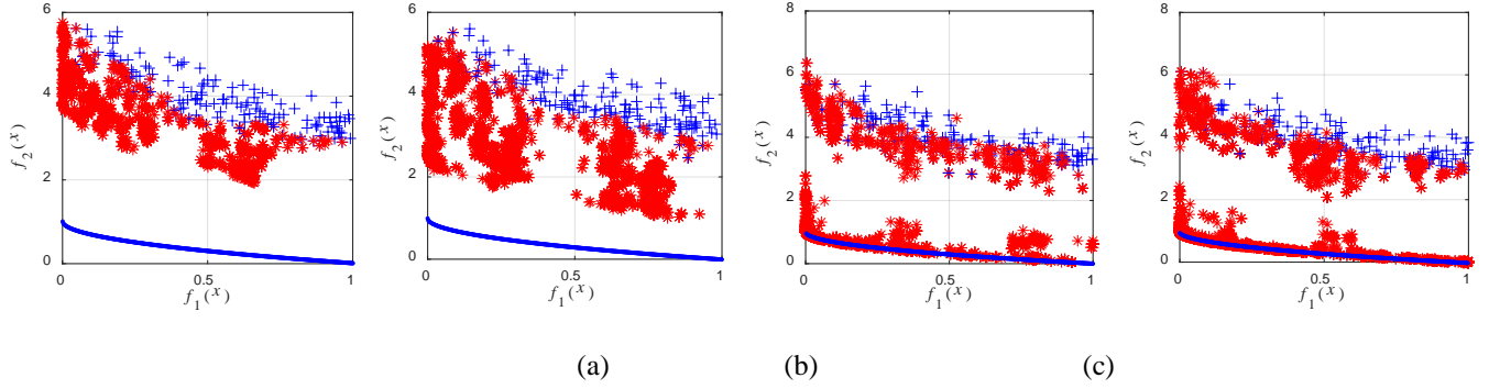
Fig. 1. Nondominated solution sets of objective function f_1(x) and f_2(x) found on the ZDT1 problem. (a) from the 1th to the 10th iteration–HEIA. (b) from the 1th to the 20th iteration–HEIA. (c) from the 1th to the 10th iteration–AUDHEIA. (d) from the 1th to the 20th iteration–AUDHEIA
