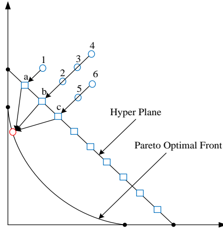
Fig. 3. Mapping of individuals on a Hyperplane.
