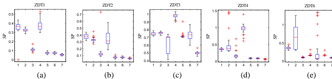
Fig. 9. Box-plots of the SP results obtained by AUDHEIA on (a) ZDT1, (b) ZDT2, (c) ZDT3, (d) ZDT4, and (e) ZDT6. (1, 2, 3, 4, 5, 6, and 7 in the horizontal axis stand for NSGAII, SPEA2, AbYSS, MOEA/D, SMPSO, HEIA and AUDHEIA, respectively.)
