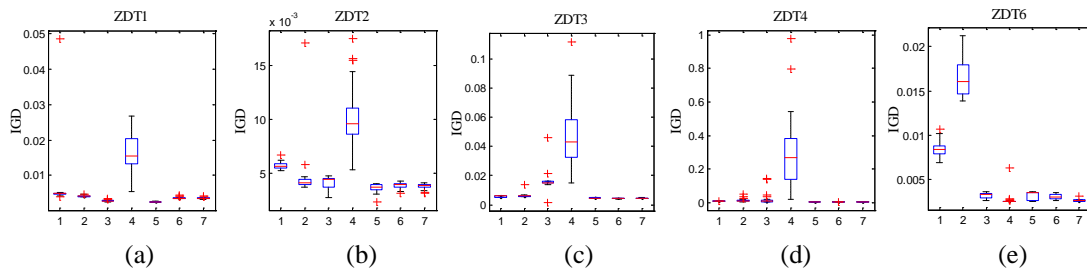
Fig. 8. Box-plots of the IGD results obtained by AUDHEIA on (a) ZDT1, (b) ZDT2, (c) ZDT3, (d) ZDT4, (e) ZDT6. (1, 2, 3, 4, 5, 6 and 7 in the horizontal axis stand for NSGAII, SPEA2, AbYSS, MOEA/D, SMPSO, HEIA, and AUDHEIA.)
