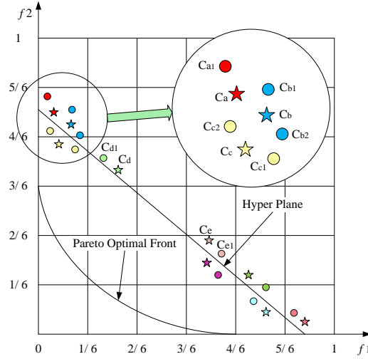
Fig. 4. The distribution of the population
