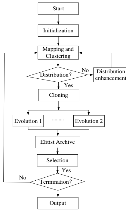
Fig. 2. Proposed framework of AUDHEIA.
