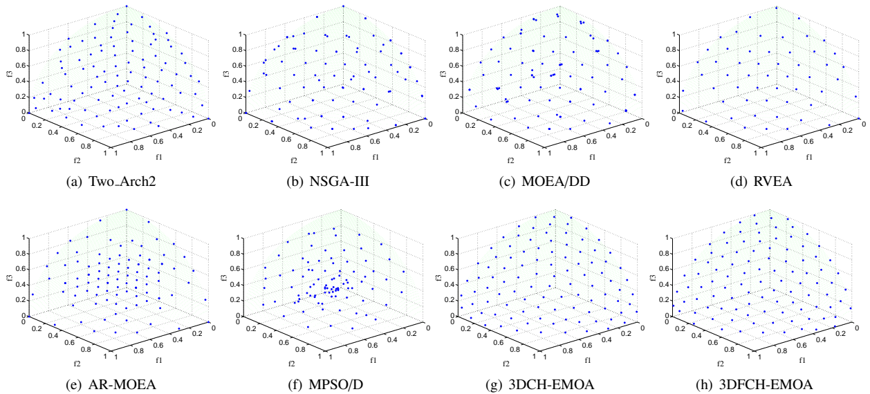
Figure 5: Experimental results of the frontal solutions (for single run) obtained by each algorithm on ZED1 test function in f_1 - f_2 - f_3 space
