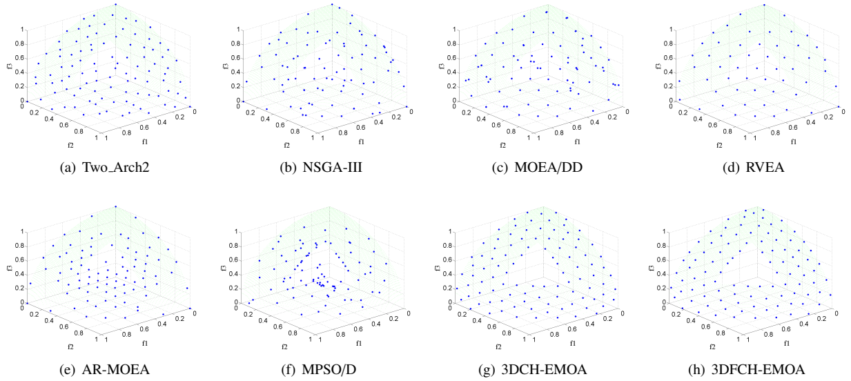
Figure 6: Experimental results of the frontal solutions (for single run) obtained by each algorithm on ZED2 test function in f_1 - f_2 - f_3 space
