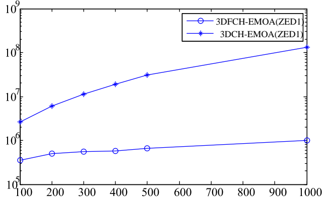
Figure 11: Comparison of execution times of 3DFCH-EMOA and 3DCH-EMOA on ZED1 test function obtained by 30 independent trials with different population sizes
