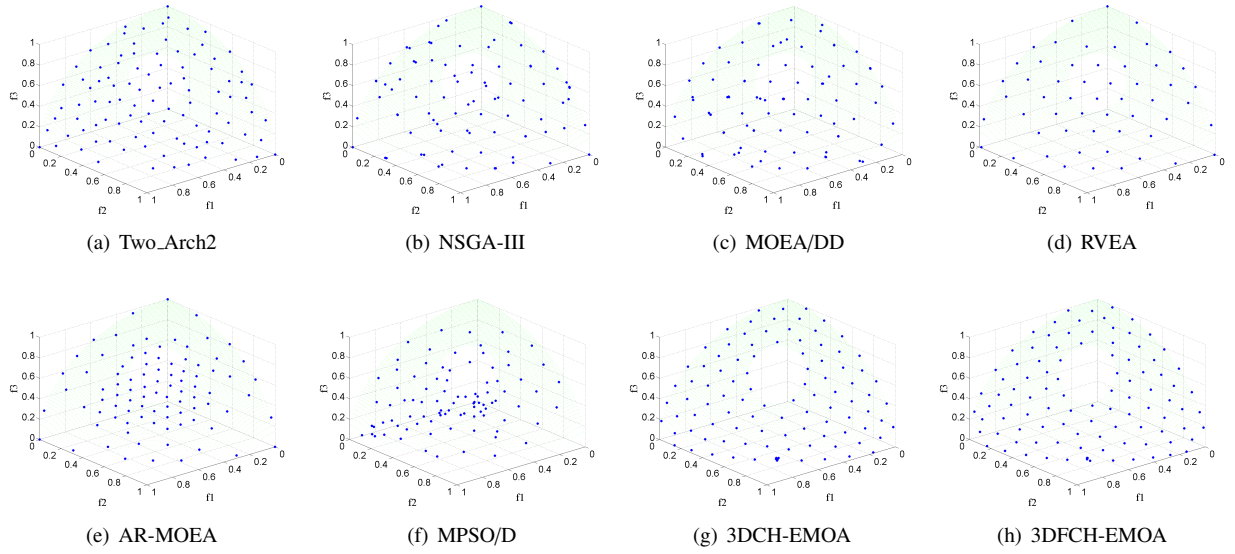
Figure 7: Experimental results of the frontal solutions (for single run) obtained by each algorithm on ZED3 test function in f_1 - f_2 - f_3 space
