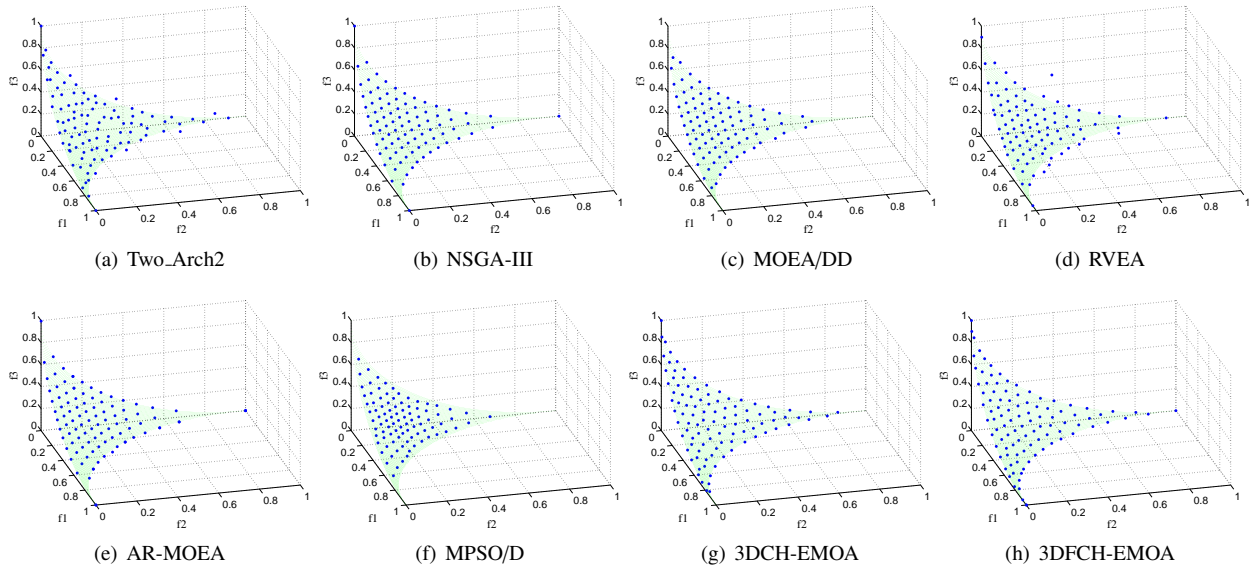
Figure 8: Experimental results of the frontal solutions (for single run) obtained by each algorithm on ZEJD1 test function in f_1 - f_2 - f_3 space
