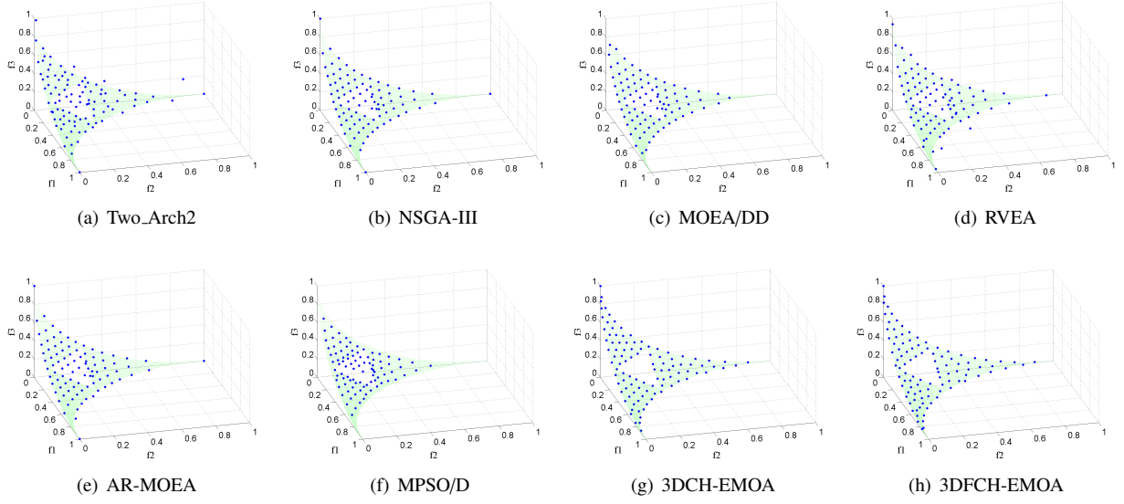
Figure 9: Experimental results of the frontal solutions (for single run) obtained by algorithms on ZEJD2 test function in f_1 - f_2 - f_3 space
