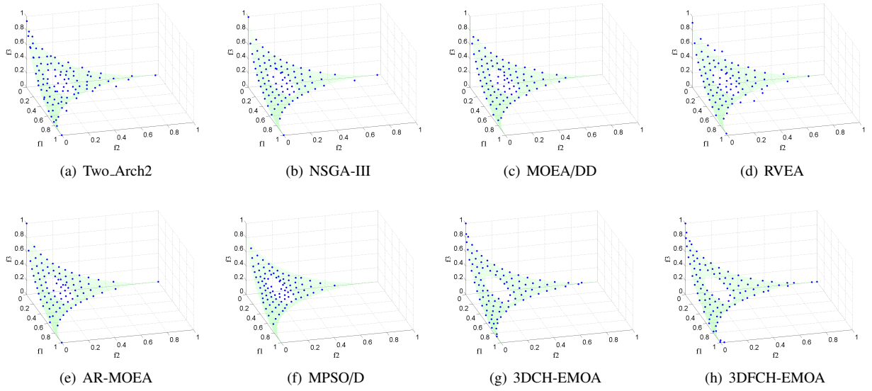
Figure 10: Experimental results of the frontal solutions (for single run) obtained by each algorithm on ZEJD3 test function in f_1 - f_2 - f_3 space
