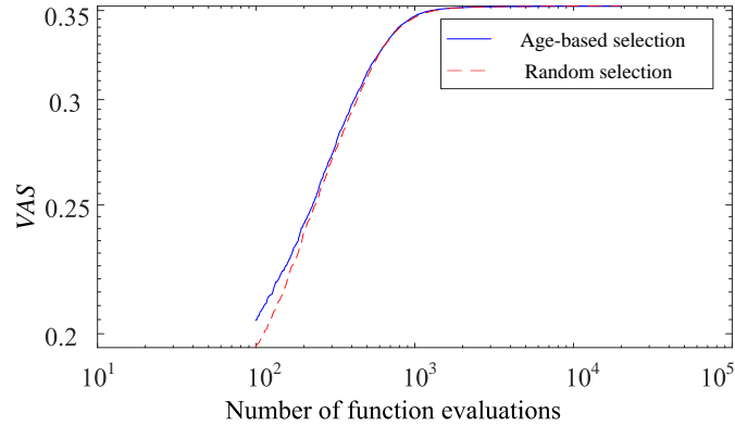
Figure 12: Average VAS of age-based selection and random selection of 3DFCH-EMOA on ZED1 test function
