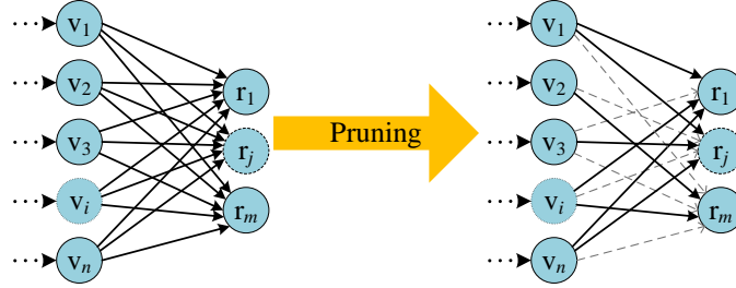
Figure 13: The diagram of neural networks pruning.
