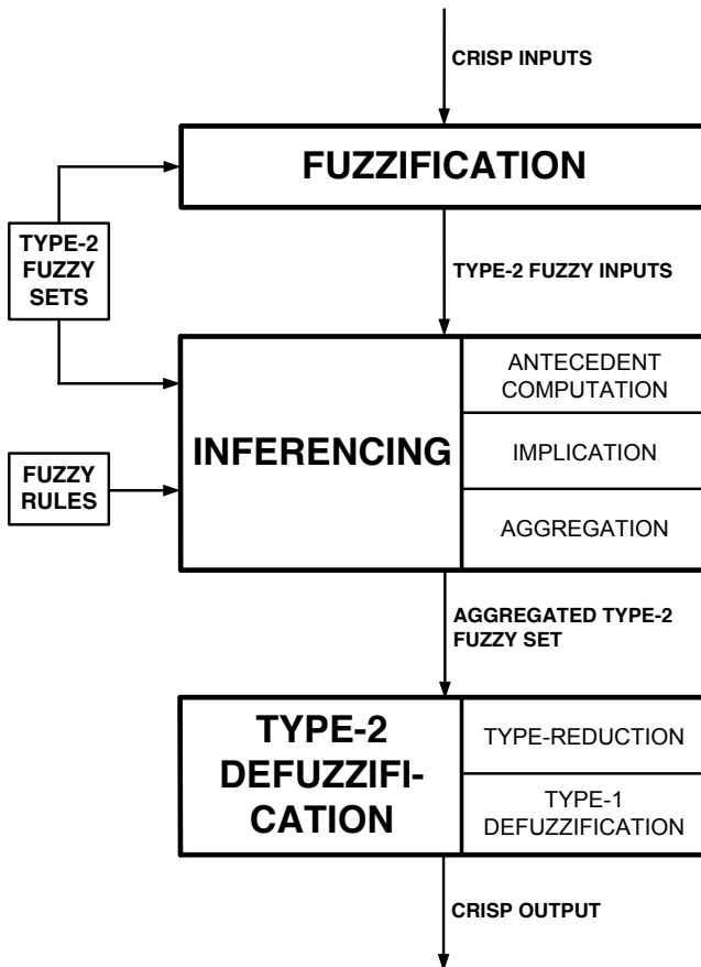
Figure 1: Mamdani-style Type-2 FIS.
