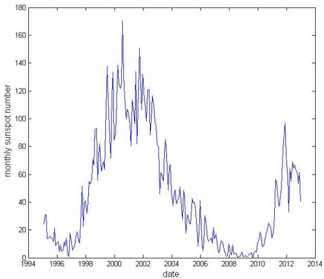
Figure 3: Number of sunspots recorded on a monthly basis between 1994 and 2013.
