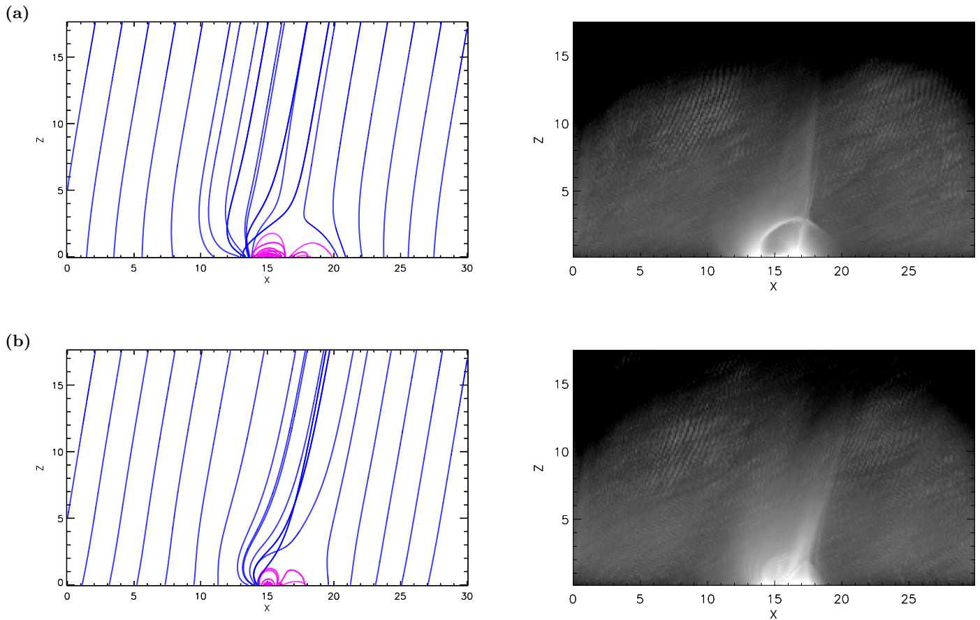
Figure 10. (a) emergence and (b) cancellation images viewed in the xz -plane, at t = 25 time steps. Left: closed (magenta) and open (blue) magnetic field lines; right: logarithm of LOS-integrated current. Movies of this Figure are available in the online version.
