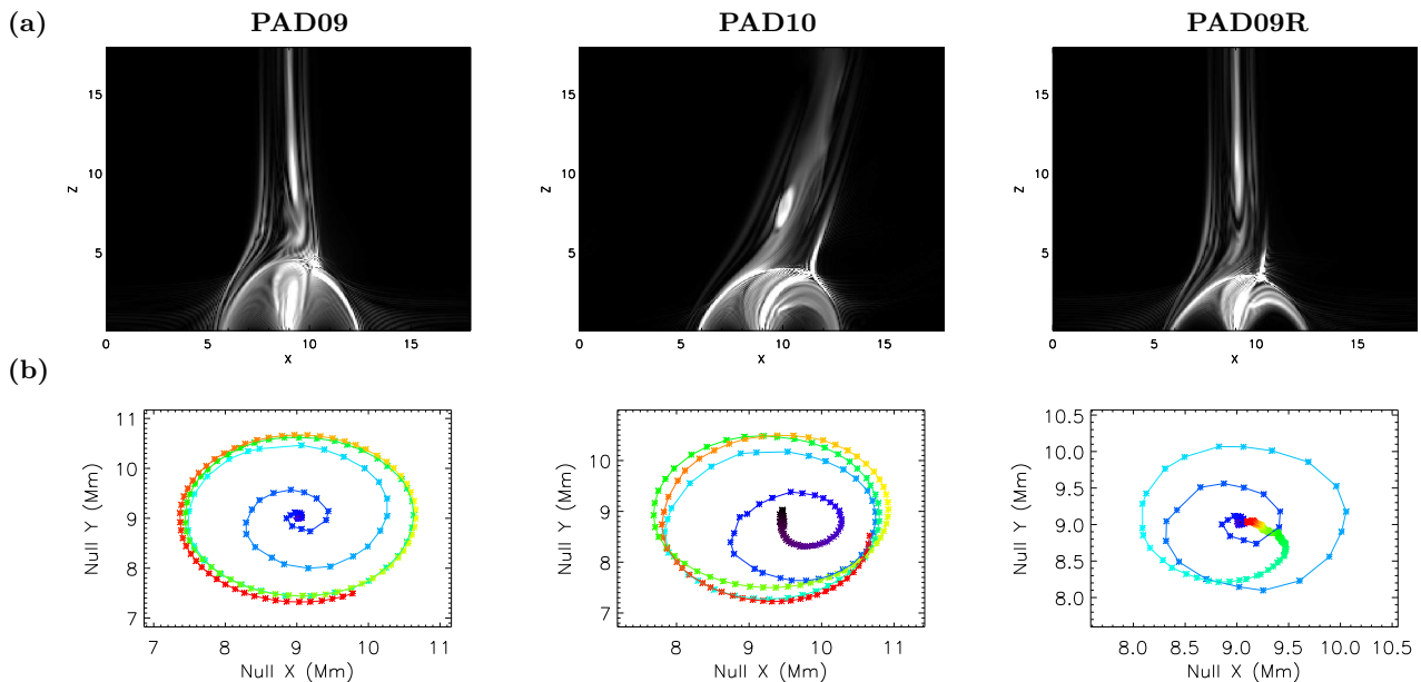
Figure 5. Plots for PAD09 (left), PAD10 (centre) and PAD09R (right). (a) |j|/|B| , viewed in the xz -plane at y = 9 Mm, at t = 70 time steps (1.4 rotations). (b) xy path of magnetic null point in time from t = 0 (black) to t = 200 (red) time steps. Movies of (a) are available in the online version.
