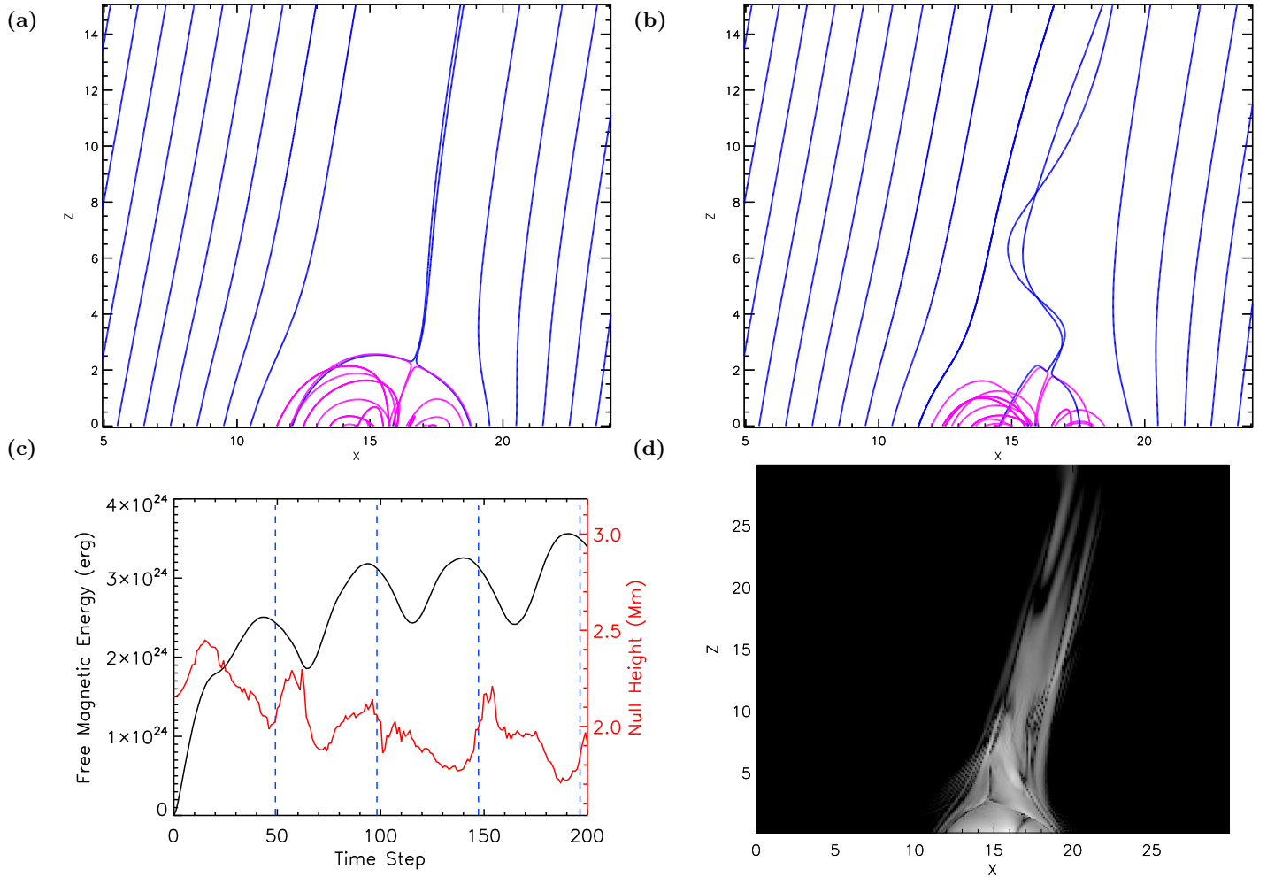
Figure 6. CIRC: (a) and (b) Closed (magenta) and open (blue) magnetic field lines viewed in the xz -plane at y = 9 Mm, at t = 30 (0.6 rotations) and t = 120 time steps (2.4 rotations). (c) Free magnetic energy (black) and height of null point (red) as a function of time. (d) Logarithm of current, viewed in the xz -plane at y = 15 Mm, at t = 120 time steps (2.4 rotations). Movies for (a)/(b) and (d) are available in the online version.
