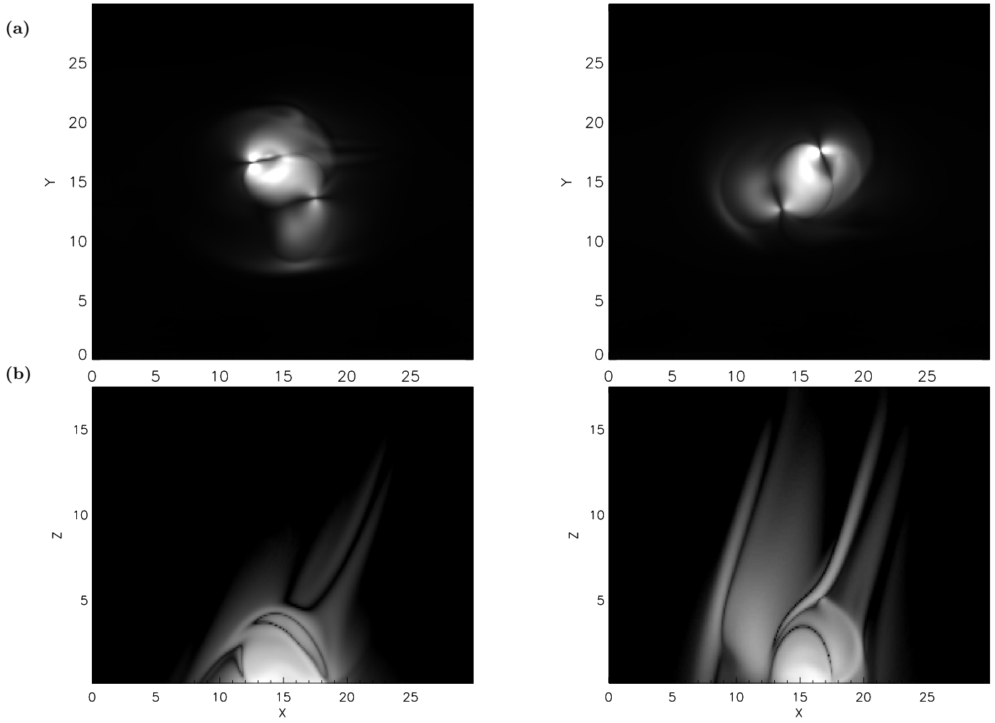
Figure 8. FLYBY1 (left) and FLYBY2 (right): (a) LOS-integrated current in the xy - plane and (b) logarithm of current in the xz -plane at y = 15 Mm, at t = 50 time steps. Movies of (a) are available in the online version.
