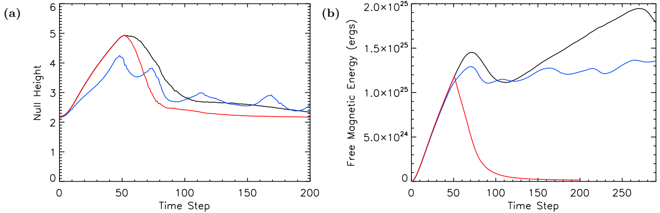
Figure 4. (a) Height of magnetic null point and (b) free magnetic energy as a function of time for PAD09 (black), PAD10 (blue) and PAD09R (red).
