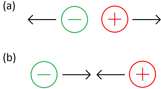
Figure 2. Two of the photospheric set-ups for this study: (a) emergence and (b) cancellation.
