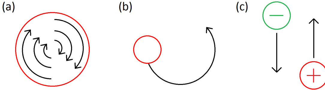
Figure 1. Three of the photospheric set-ups for this study: (a) a positive polarity with approximately solid-body rotation; (b) a positive polarity moving in a circle; (c) flyby.
