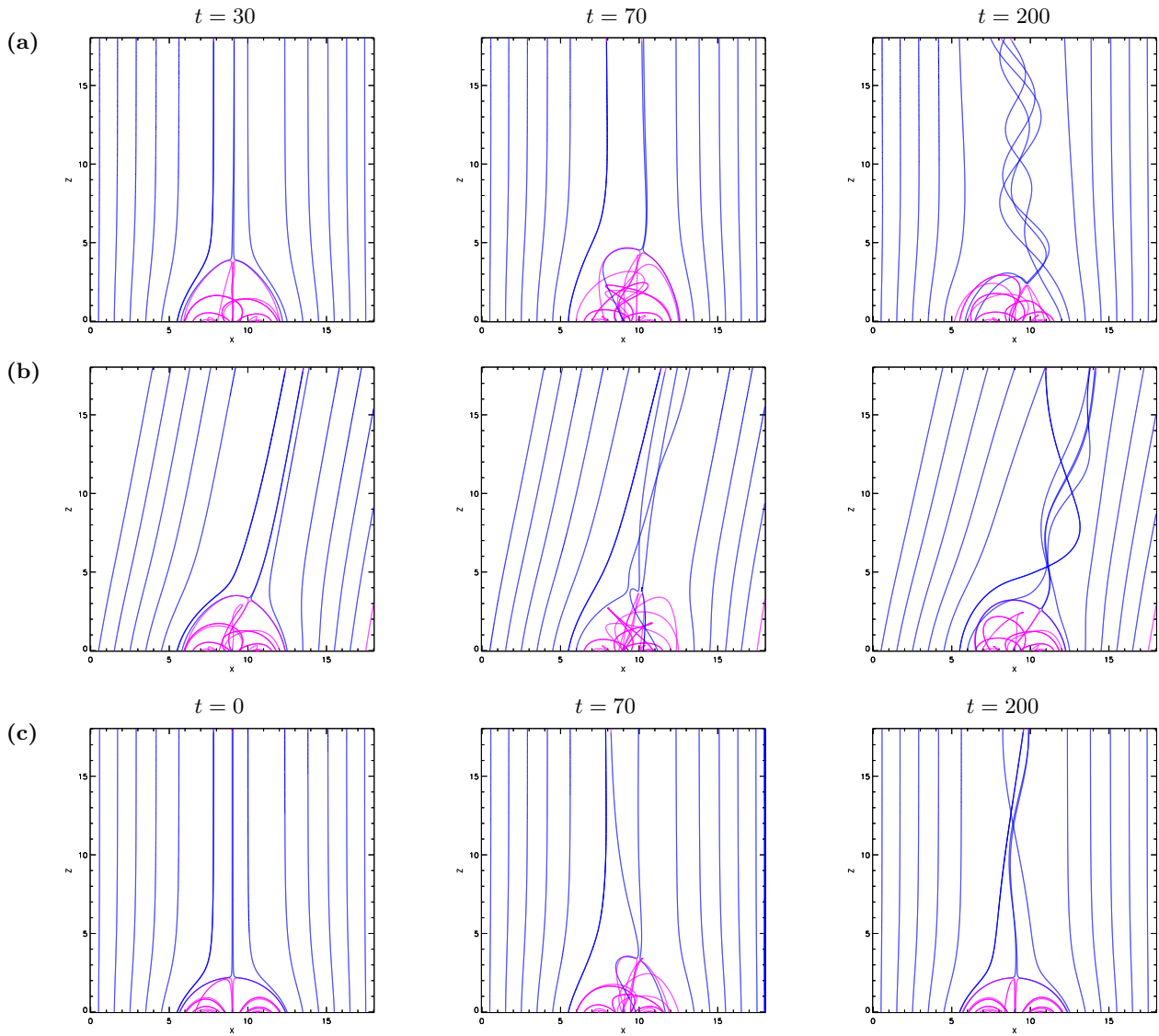
Figure 3. Closed (magenta) and open (blue) magnetic field lines viewed in the xz -plane at y = 9 Mm, for (a) PAD09, (b) PAD10 and (c) PAD09R. For (a) and (b), plots are shown at t = 30 time steps (left, 0.6 rotations), t = 70 (centre, 1.4 rotations - after onset of kink) and t = 200 (right, 4 rotations). For (c), PAD09R, plots are shown at t = 0 time steps (left), t = 70 (centre) and t = 200 (right). Note that PAD09 and PAD09R are identical at t = 0 and t = 30 timesteps, so plot (a) left and (c) left apply to both simulations. Movies of these Figures are available in the online version.
