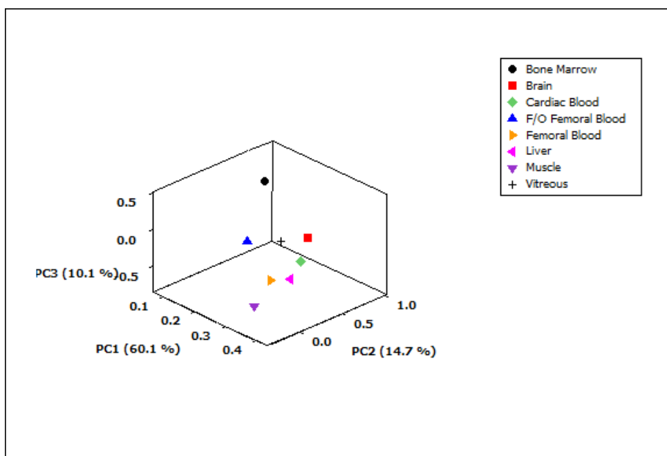
Fig 3: 3D scatterplot for morphine concentration with cardiac blood results below 0.3 mg/L
