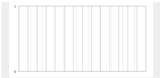
Figure 9: A spectral plot of two non-coincident impulse trains shows a more complex relationship. There is variability in the spacing between components and some clustering, leading to beating. The uniform magnitude of the components makes it very difficult to identify discrete pitches.
