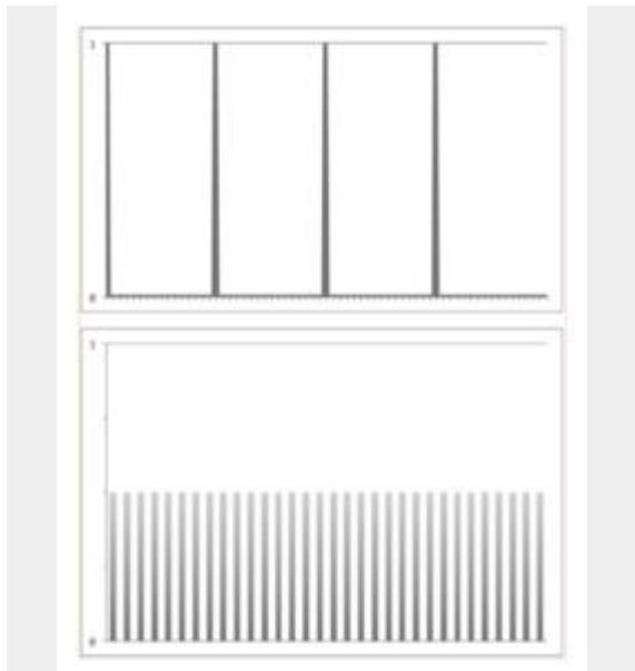
Figure 6 – Outputting an impulse train generates a signal whose frequency spectrum contains an equal amount of energy across all harmonics. The top plot here shows a time domain representation of the sound, showing a series of impulses separated by silence. The lower plot shows a frequency domain representation of the same sound, which has its energy distributed equally across all of its harmonics.
