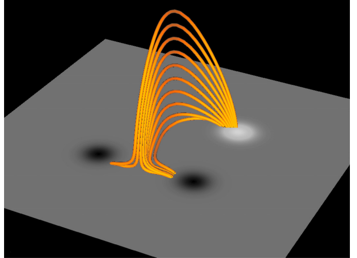
Fig. 1. Magnetic field lines of the linear force-free region are displayed in orange. A magnetogram of B_z is given at the base to indicate the positions of the sources.
