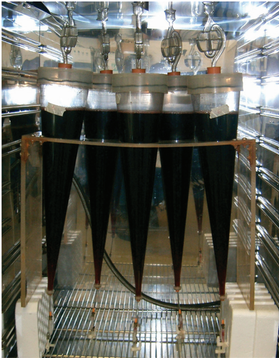
Figure 6 Imhoff conical vessels used in small-scale wine fermentation. Wine yeast strains were grown in graduated conical vessels (1 L, cone angle 74°) made of polycarbonate and closed with fermentation locks. Cones were washed previously with nitric acid, ddH 2 O, EDTA (as described in Materials and methods) and filled with grape juice. Yeast cells were inoculated at initial cell density of 12 \times 10^6 cells/mL and fermentation was carried out at 25 °C for five days.
