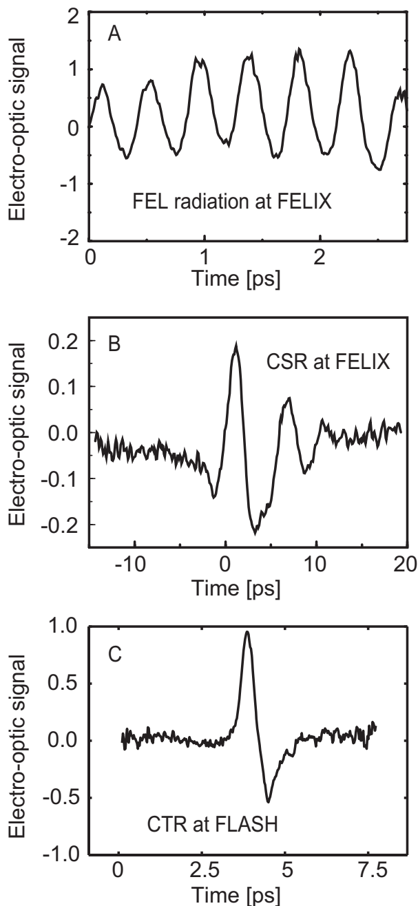
Figure 3: Single-shot electro-optic measurements of (A) FEL radiation, (B) CSR radiation and (C) CTR radiation. The leading edges of the pulses are on the left. Note the different time scales. See text for details.
