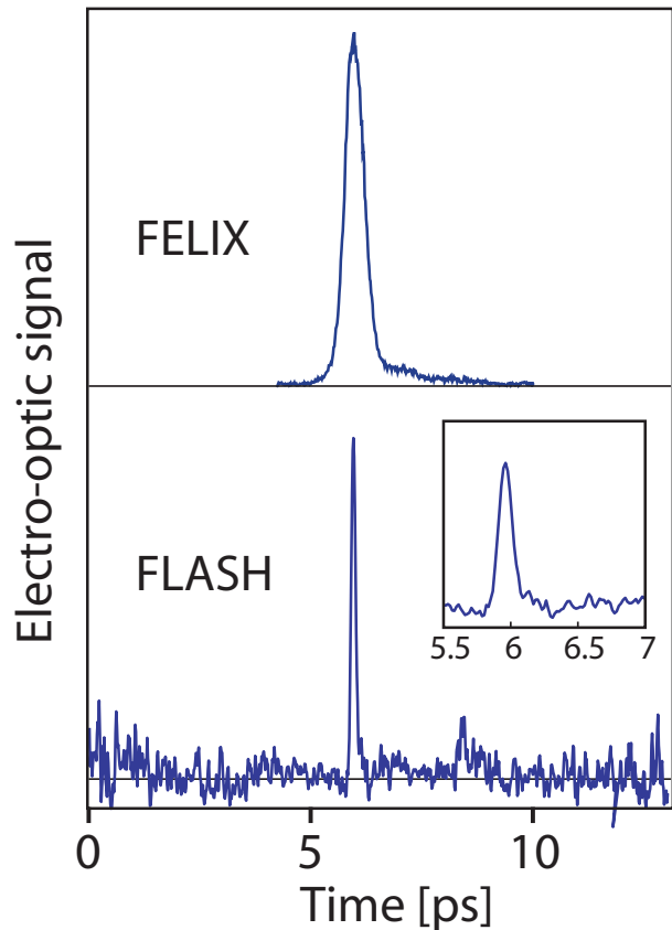
Figure 2: (color) Single-shot electro-optic bunch profile measurements recorded at FELIX (top) and FLASH (bottom). See text for details.
