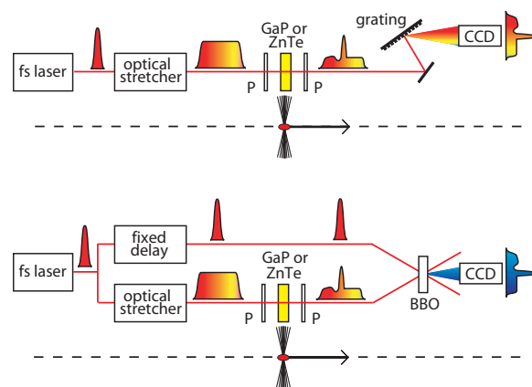
Figure 1: (color) Single-shot techniques for measuring the longitudinal electric field profile of single electron bunches using electro-optic encoding with spectral decoding (top) and temporal decoding (bottom).
