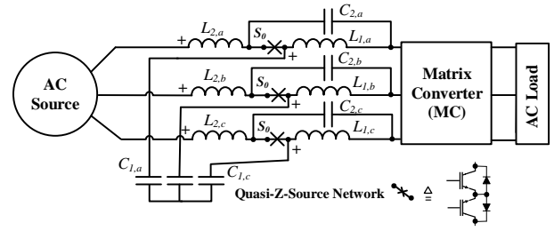
Fig. 10. Quasi-Z-source MC [92]
