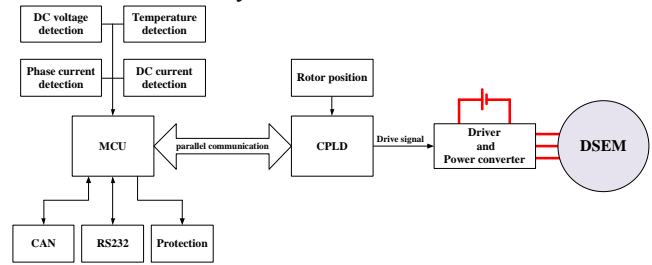
Fig. 22. Hardware platform diagram.
