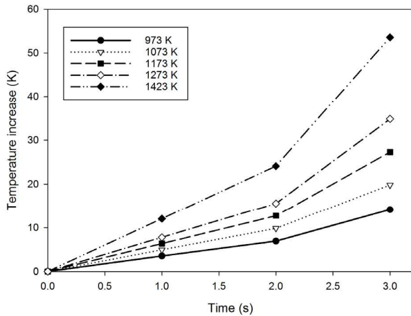
Fig. 10 Temperature increase of the radiation shield.
