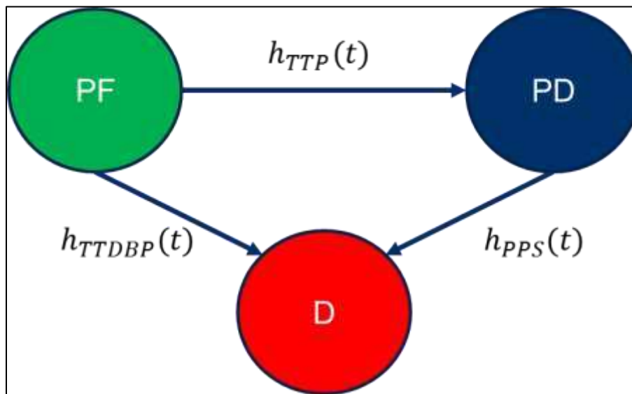
Figure 5. Structure of the three-state model for PFS fitted to the study data and used in simulations.
