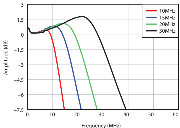
Fig. 1. Gain vs. Frequency of Commercial AFE LPF at Different Cut-off Frequencies (Adapted From [5])
