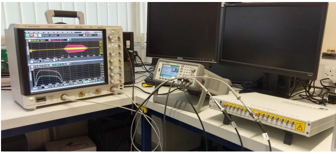
Fig. 4. Experimental Setup for Measuring UARP AFE Frequency Response
