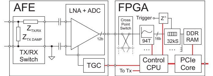
Fig. 3. Diagram of Rx Portion of UARP System Architecture
