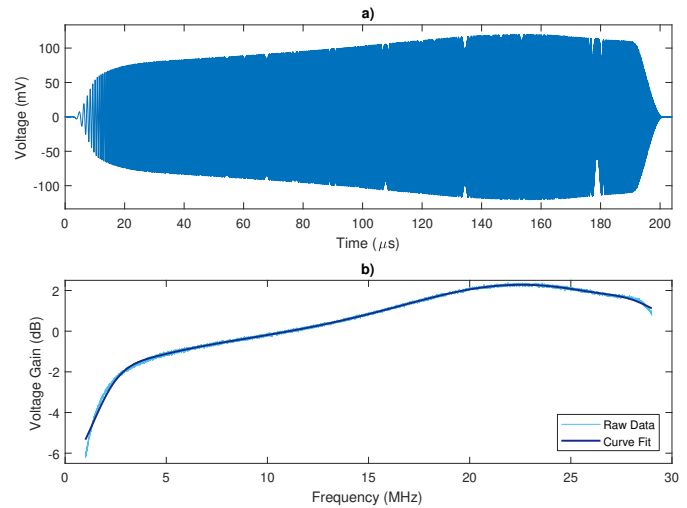
Fig. 6. Measured Voltage (a) and FFT (b) of Gain Frequency Response of UARP AFE with No Correction
