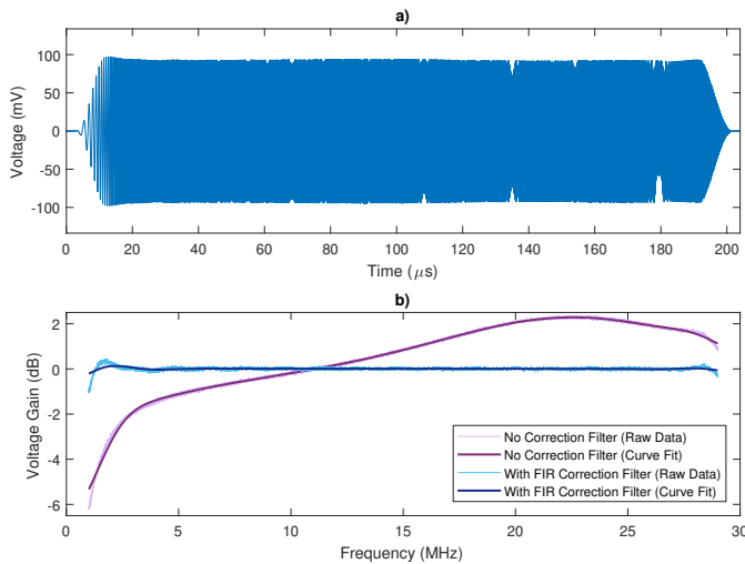
Fig. 7. Measured Voltage (a) and FFT (b) of Gain Frequency Response of UARP AFE with FIR Filter Correction Enabled
