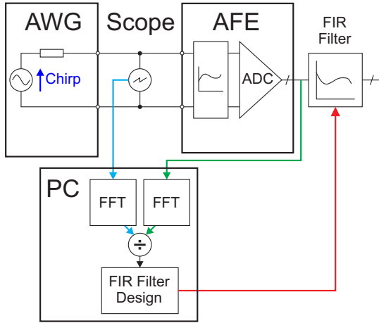
Fig. 2. Setup for Measuring Distortion of Analog Front End and Calculating Required Normalisation Filter Response
