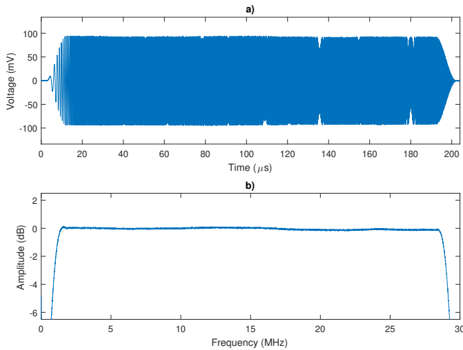
Fig. 5. Measured Voltage (a) and FFT (b) of Chirp Test Signal with 15 MHz Centre Frequency and 28 MHz Bandwidth Captured using Oscilloscope
