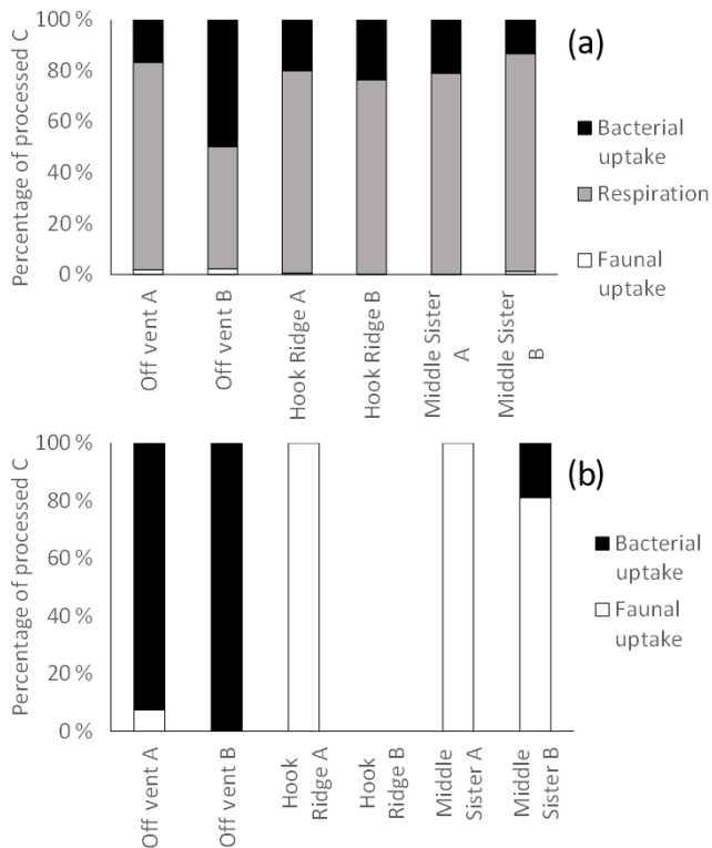
Figure 7. Distribution of biologically processed C between processes for the (a) algae addition experiments and (b) bicarbonate addition experiments. The absence of data represents the combination of the lack of sample and an undetectable faunal ^{13}\text{C} uptake.
