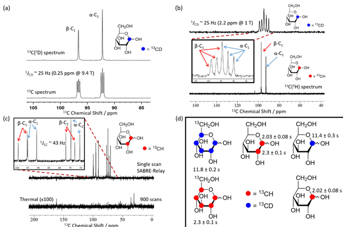
Figure 4 - SABRE-Relay hyperpolarized ^{13}\text{C} NMR spectra. (a) ^{13}\text{C}\{^2\text{H}\} NMR spectrum (top) and a ^{13}\text{C} NMR spectrum (bottom) of 2.5 mg (21.1 mM) of mM D-glucose-1,2- ^{13}\text{C}_1 , d_1 (structure inset) with 4.8 mM of 3 and 23.8 mM benzyl- d_7 -amine in 0.65 mL DCM- d_2 : DMF (1.6:1) measured at 9.4 T. (b) Corresponding results showing a ^{13}\text{C} spectrum of D-glucose-1,2- ^{13}\text{C}_1 , d_1 (top) and a ^{13}\text{C}\{^1\text{H}\} spectrum of D-Glucose-1,2- ^{13}\text{C}_1 (bottom) measured at 1 T. The inset spectrum reflects the boxed region of interest and highlights the presence of two isomers whose signals overlap. (c) Hyperpolarized (top) and 900 scan thermal reference scan (bottom, \times 100 scaling) for a 21.1 mM D-glucose-1,2- ^{13}\text{C}_2 sample with 4.8 mM of 3 and 23.8 mM benzyl- d_7 -amine in DCM- d_2 :DMF (1.6:1) (0.6 mL) acquired at 1 T. The inset of (c) shows the region of interest and demonstrates that both isomers can be distinguished at 1 T. (d) Structures of the glucose variants used in this study along with their corresponding hyperpolarized T_1 values at 1 T. In the case of the ^{13}\text{C}_6 variants all peaks were analyzed together due to spectral overlap.
