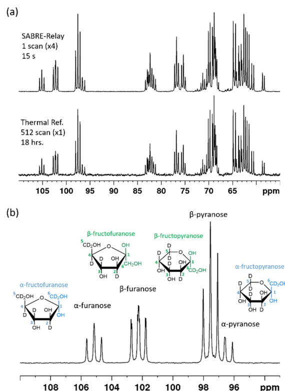
Figure 8 - (a) SABRE-Relay hyperpolarized ^{13}\text{C} ( ^2\text{H} ) NMR spectrum of 19.9 mM of ^{13}\text{C}_6\text{-}d_7 -fructose with 23.8 mM benzyl- d_7 -amine and 4.8 mM [IrCl(COD)](IMes) of d_{22}\text{-}5 in a 0.65 ml DCM- d_2 :DMF (1.6:1) mixture measured at 9.4 T (top spectrum) with the corresponding thermal reference, averaged over 512 scans (bottom spectrum, 18 hrs.). (b) Expansion of (a) to highlight the different isomeric forms indicated by their C-2 resonances.
