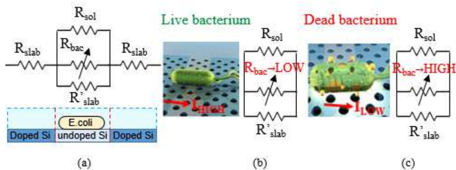
Fig. 4. Equivalent electrical circuit of (a) the cross-section of the electro-photonic device with (b-c) a focus in the region of trapping site, with R_{slab}' the resistance of the PhC silicon slab, R_{sol} the resistance of the surrounding solution, R_{bac} the resistance associated to the bacterium (b) R_{bac} is low when the bacterium is live and (c) high when the external membrane is disrupted by the antibiotics, which corresponds to high and low values of current, respectively.
