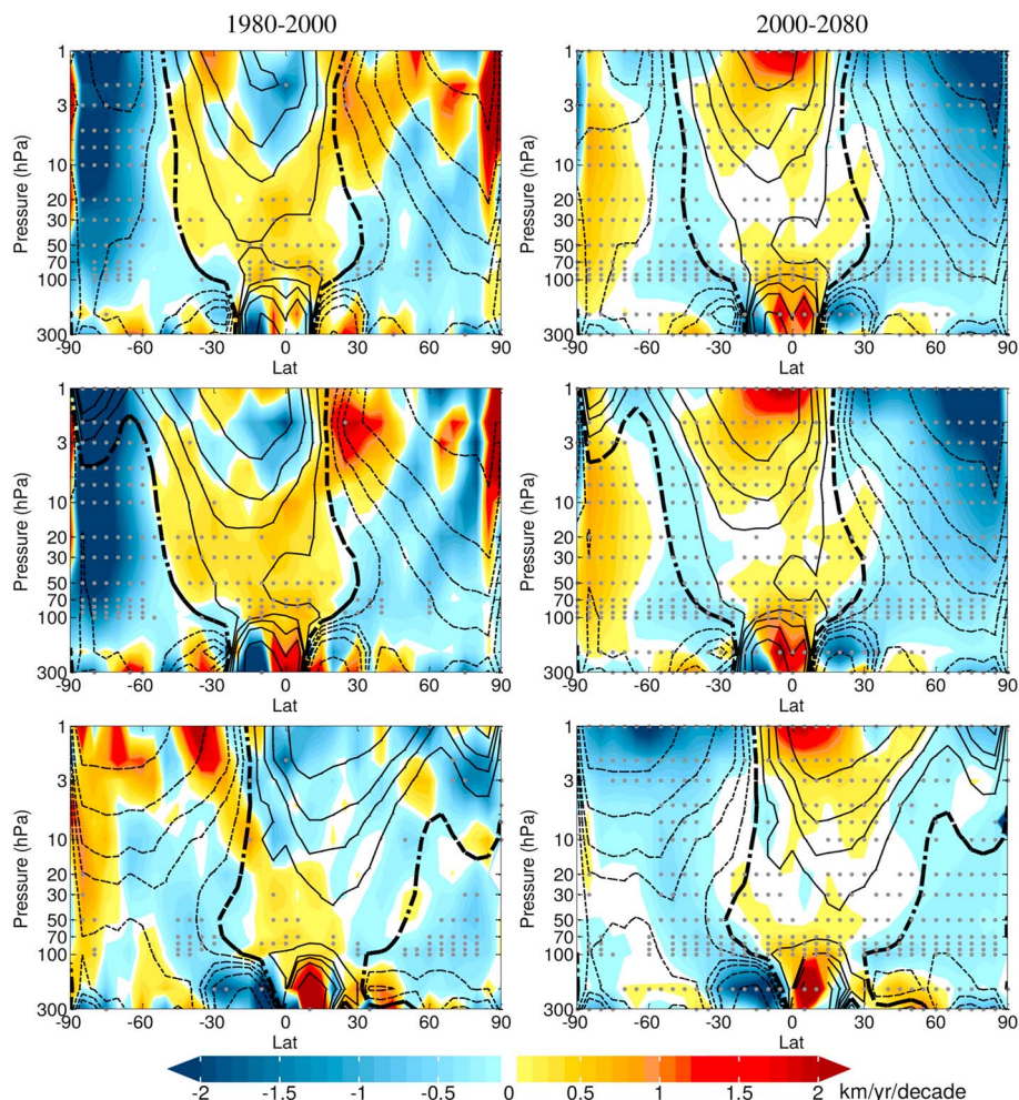
Figure 3. Past (left) and future (right) multimodel mean, zonal mean \bar{w}^* trends (shading) in the annual (top row), December–February (middle row), and June–August (bottom row) means. The black contours show the corresponding climatology, with contour lines at -100, -50, -30, -20, -10, 0, 10, 20, 30, 50, and 100 km/year, positive in solid, zero in dash dotted, and negative in dashed. The gray stippling shows where trends are significant at the 95% interval, using a two-tailed t test.
