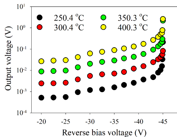
Figure 2. Output voltage of InGaAs APD thermometer as a function of reverse bias voltage for target temperatures of 250.4 ^{\circ} C, 300.4 ^{\circ} C, 350.3 ^{\circ} C and 400.3 ^{\circ} C.
