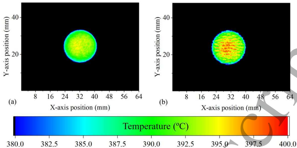
Figure 7. Thermal images of a 20 mm diameter target aperture placed in front of a furnace at a temperature of 395 °C, using (a) InGaAs APD and (b) InGaAs photodiode based scanners.
