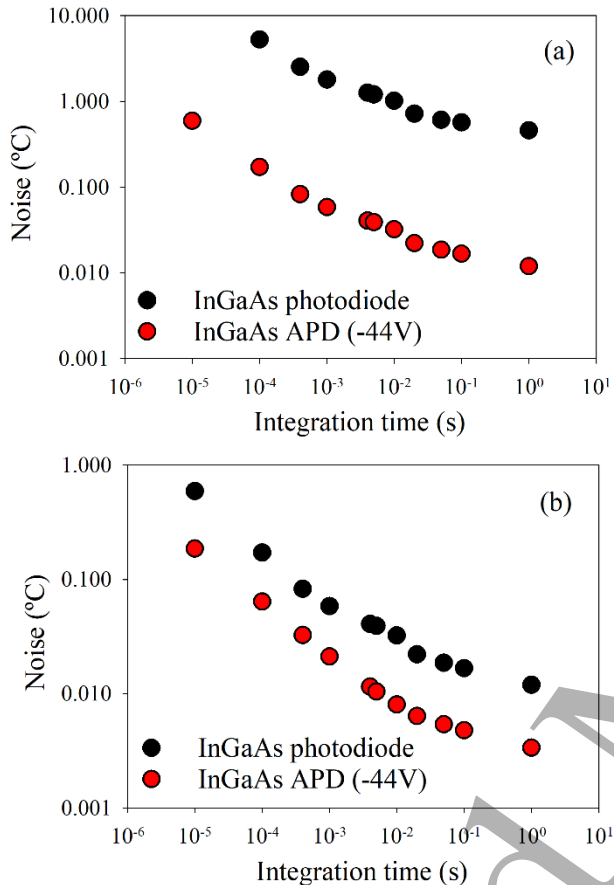
Figure 6. Noise of InGaAs photodiode and InGaAs APD thermometers as functions of integration time. Target temperatures of (a) 250.4 °C and (b) 400.3 °C.
