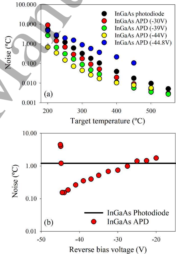
Figure 5. (a) Noise of InGaAs photodiode and InGaAs APD thermometers with target temperature. (b) Noise as a function of InGaAs APD reverse bias voltage for a target temperature of 250.4 °C, compared with the unbiased InGaAs photodiode. Integration time of 5 ms.
