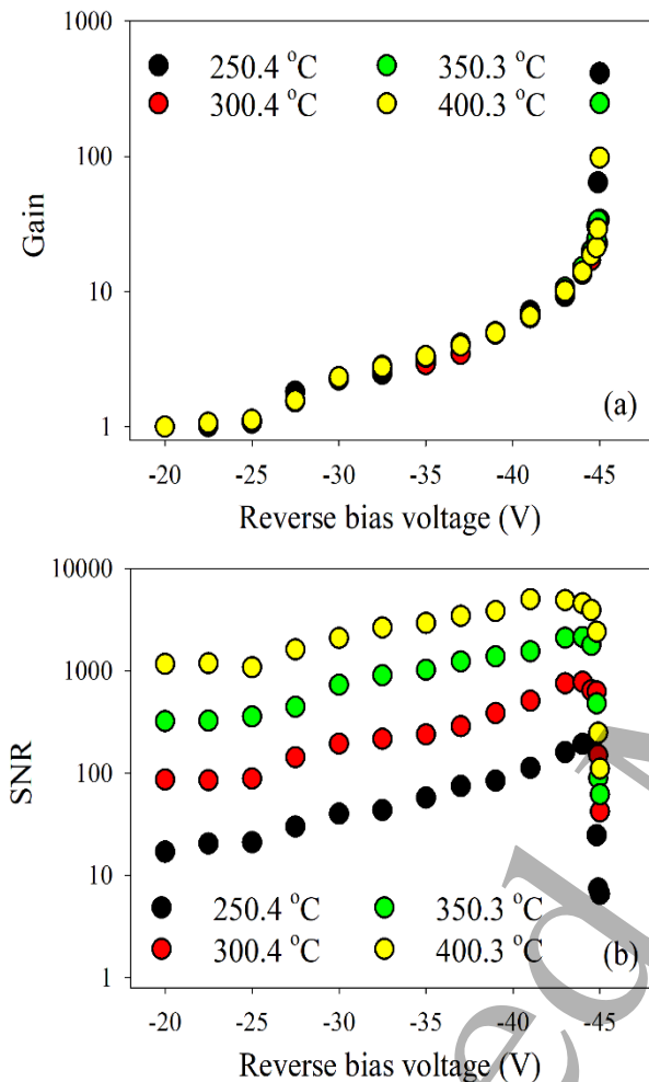
Figure 3. (a) APD gain and (b) SNR with 5 ms integration time for InGaAs APD thermometer as a function of reverse bias voltage for target temperatures of 250.4 °C, 300.4 °C, 350.3 °C and 400.3 °C.
