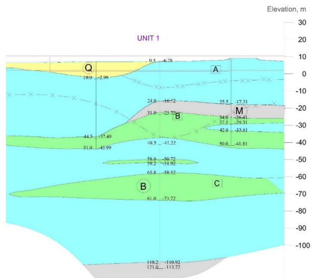
Fig. 3: Engineering geological cross-section under NPP main building.
