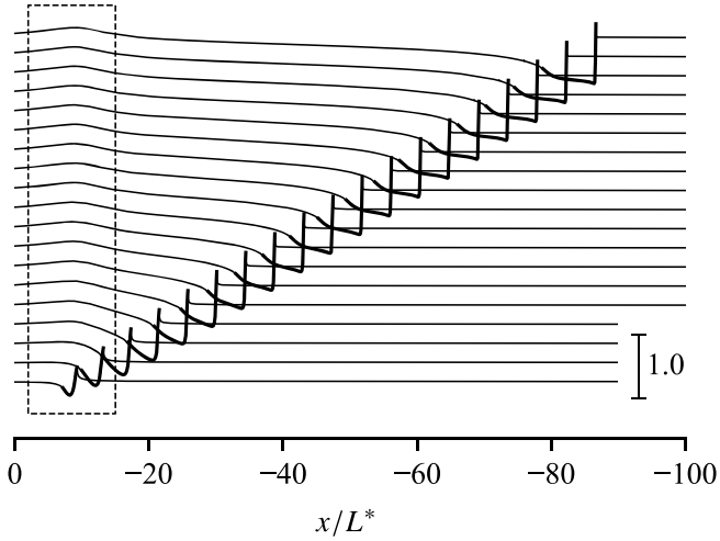
Figure 10. Stress buildup due to the transition to an expanding pulse. Simulation run using \tau_b/\tau_0 = 0.77 , and a positive stress perturbation located at x = 0 . (a) Snapshots of stress profiles. Thick lines highlight the slipping patch. Box highlights the stress buildup around the transition point. (b) Evolution of the maximum stress perturbation behind the pulse and maximum slip perturbation as a function of time.
