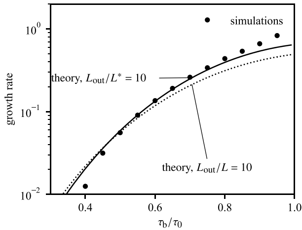
Figure 11. Comparison of perturbation growth rates from numerical simulations (dots) and theoretical estimates based on the slip pulse equation of motion (solid and dotted lines). The latter are computed using the relationships \tau_{b,ss}(b) , v_{r,ss}(b) shown in Figure 3 and equation (40), with either L_{out}/L^* = 10 and L = L_{ss} (solid line) or L_{out}/L = 10 (dotted line).
