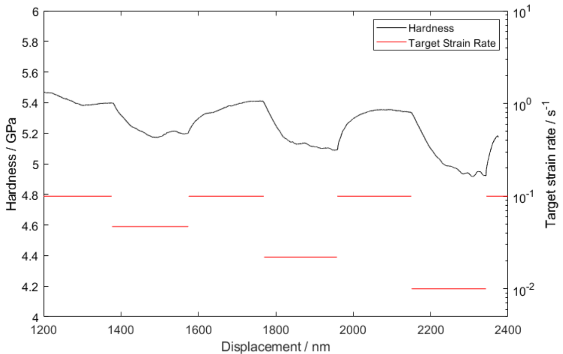
Figure 8 Hardness versus depth for strain-rate jump tests. The change in hardness corresponding with each decrease and increase in strain rate can be clearly observed. The base strain rate was 0.1 \text{ s}^{-1} with lower strain rates of 0.047 , 0.022 and 0.01 \text{ s}^{-1} .
