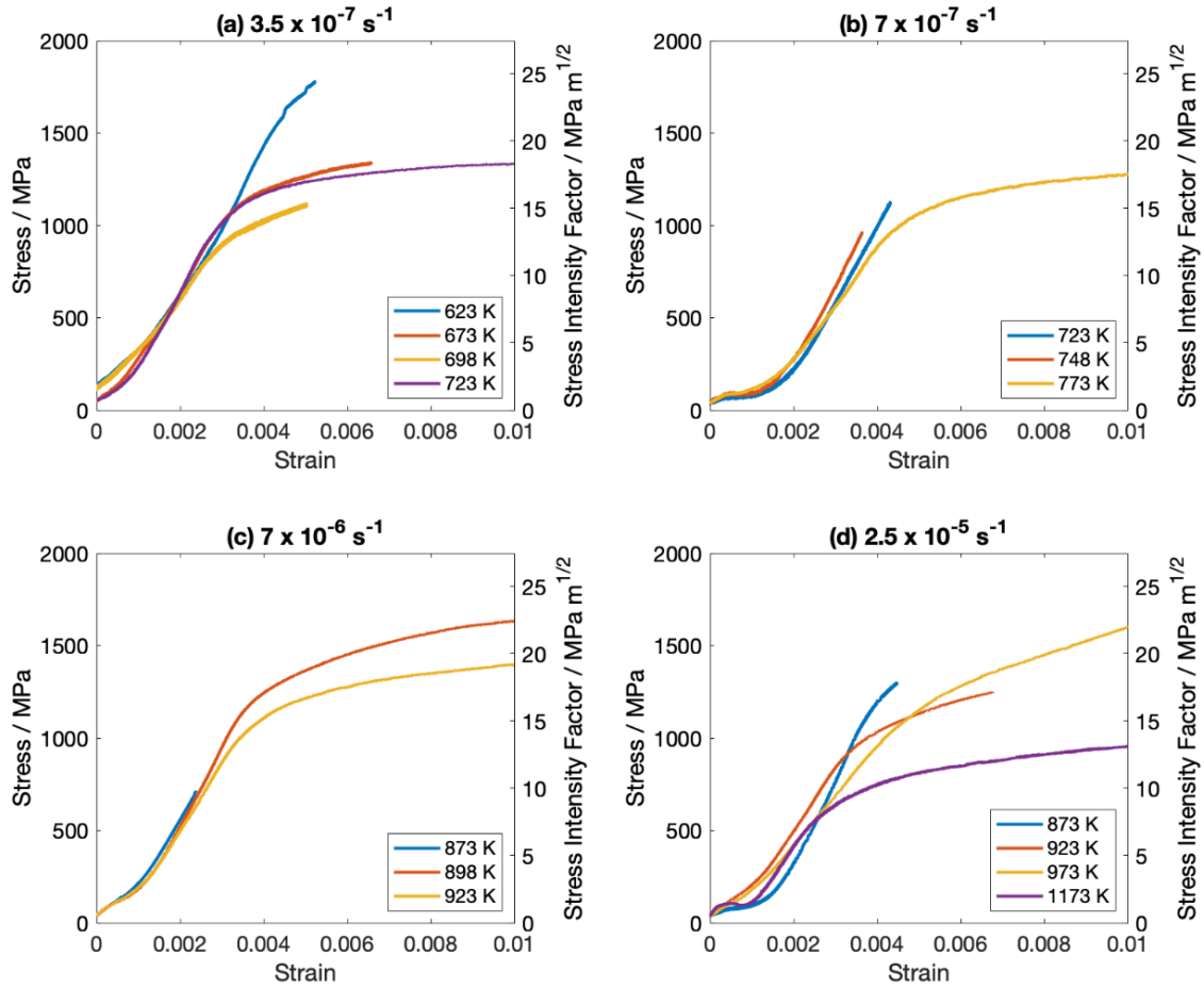
Figure 3 Four-point bending stress-strain curves for neutron-irradiated single crystal W at a range of temperatures and strain rates. The transition from brittle to ductile behaviour with increasing temperature can be clearly observed at each strain rate.
