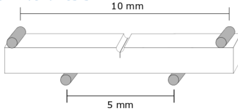
Figure 2 Geometry of four-point bend tests of 1 x 1 mm cross-section samples. The samples were loaded such that the notch and pre-cracks were on the tensile face of the specimen
