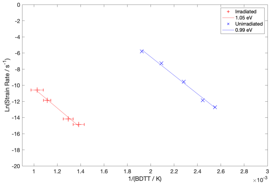
Figure 5 Arrhenius plot comparing activation energy of BDT in unirradiated W and neutron irradiated W
