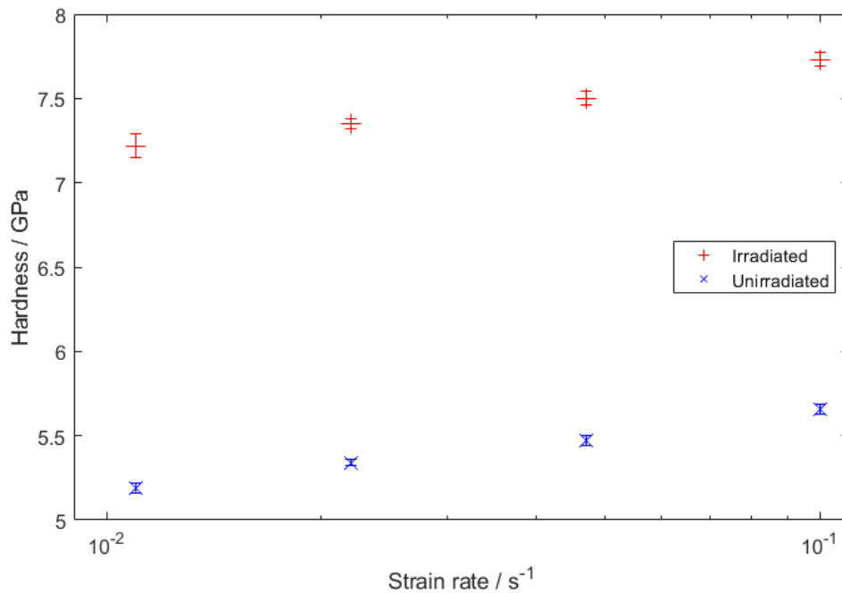
Figure 9 Results from strain rate jump tests in neutron irradiated and unirradiated tungsten single crystal, showing the increase in measured hardness depending on the applied strain rate
