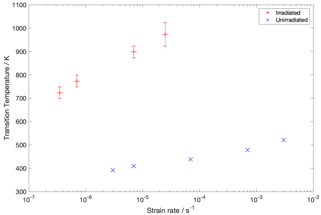
Figure 4 Comparison of BDTT at a range of strain rates for unirradiated W [7] and neutron irradiated W. Error bars were calculated as the temperature gap between highest brittle test temperature and lowest ductile test temperature
