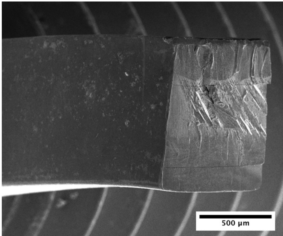
Figure 7 Low magnification image showing large ductility of neutron irradiated sample before fracture at 823 K with a strain rate of 7 \times 10^{-7} \text{ s}^{-1}
