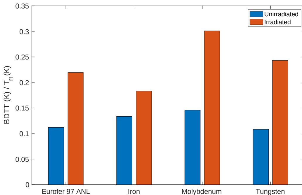
Figure 10 Increase in BDTT as a proportion of melting point in BCC metals following neutron irradiation. Eurofer 97 ANL was irradiated to 16.3 dpa at 573 K [59], molybdenum to 2.2 dpa at 782 K [60] and iron to 0.4 dpa at 678 K [61]
