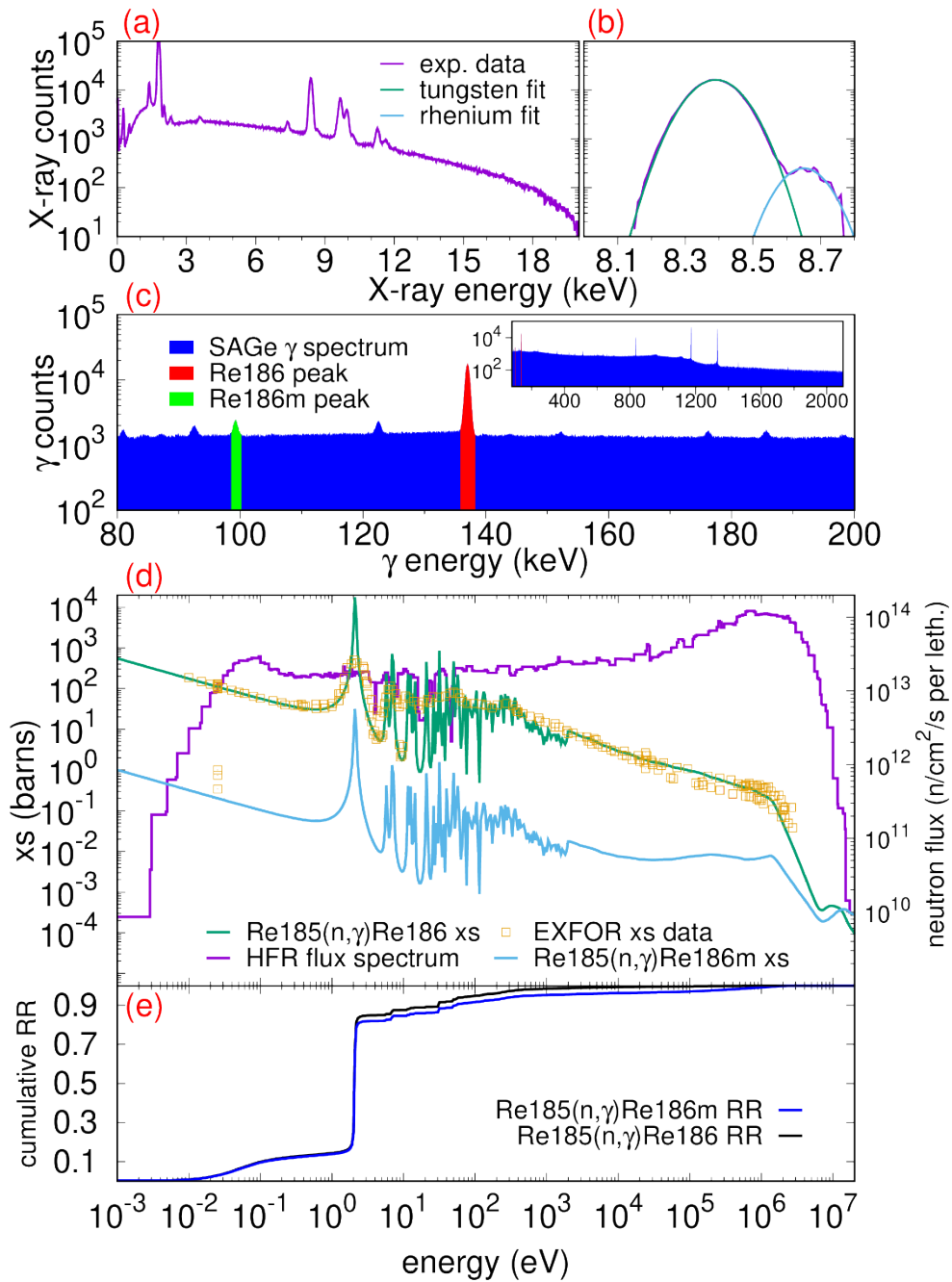
Figure 1 Transmutation and \gamma -spectroscopy analysis of the samples. a) raw EDS X-ray spectrum. b) zoomed portion of X-ray spectrum showing Gaussian fit to W-peak at \sim 8.4 keV and Re peak at 8.65 keV with the comparative areas under each curve indicating the amount of Re in the sample. Note that in (b) the data first had the background counts removed via analysis of the background in the range 8-9 keV for the data in (a). (c) \gamma -spectroscopy measurements of irradiated samples showing the full spectrum (inset) and the region below 200 keV with the peaks associated with Re186 activity highlighted. (d) Nuclear cross section (xs) data for neutron capture on Re185 for production of Re186 and its metastable state Re186m. The data is compared to the available experimental measurements from the EXFOR international database and the simulated HFR flux spectrum experienced by the samples is shown for reference using the right-hand \gamma -axis scale. "per leth." or per lethargy refers to the standard practice of dividing the flux by the logarithm of the energy bin width to remove bias caused when bins have large variation. (e) shows the cumulative reaction rate (RR) of the two neutron capture reactions under the HFR spectrum. See main text for more details.
