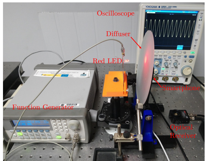
Fig. 4. Experimental setup
