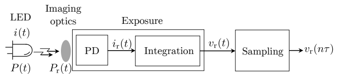
Fig. 1. The Simplified model for cameras in OCC
