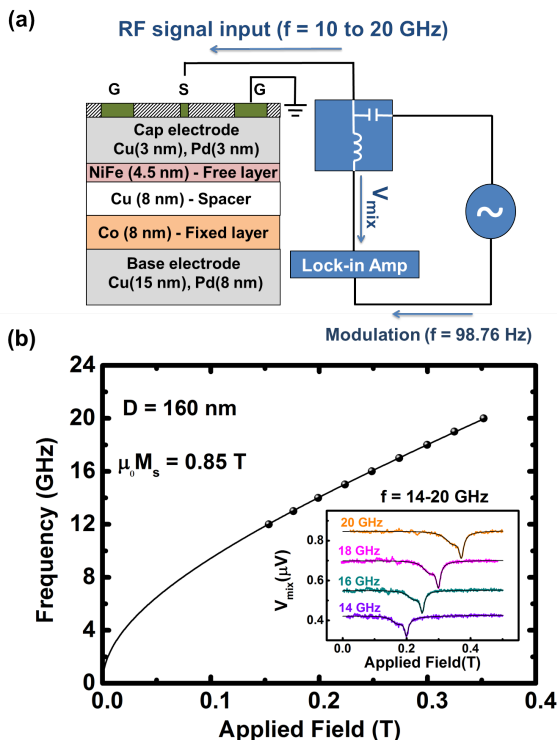
FIG. 1. (a) Schematic of the NC-STO and the measurement set-up. (b) Inset: ST-FMR spectra at four different frequencies for the D=160 nm sample. Main figure: Plot of the field position of the dominant resonance peak. The resonance fields can be well fit by the Kittel equation using \mu_0 M_s = 0.85 \pm 0.02 T for the NiFe layer.
