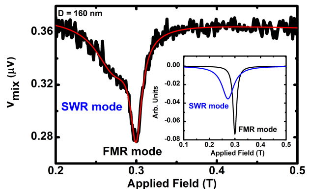
FIG. 2. Zoom-in of a representative ST-FMR spectrum of the D=160 nm sample taken at f = 18 GHz and I_{rf} = 1.3 mA, together with a fit (red line) based on two Lorentzians as described in the text. The inset shows the two individual contributions of the quasi-uniform FMR mode (black), and the spin wave resonance (blue).
