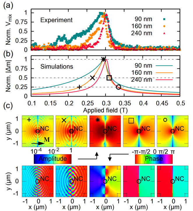
FIG. 5. (a) The normalized measured mixing voltage ( V_{mix} ) and (b) the normalized simulated magnetization precession amplitude for the three NC diameters as a function of the applied in-plane magnetic field. (c) Spatial maps of the magnetization precession amplitude (top row) and phase (bottom row) simulated for a D = 160 \text{ nm} NC diameter taken at the fields corresponding to the main peak and its 1/2 and 1/4 heights (as shown by the corresponding black symbols in (b)). Propagating spin waves are clearly seen for the two lowest fields.
