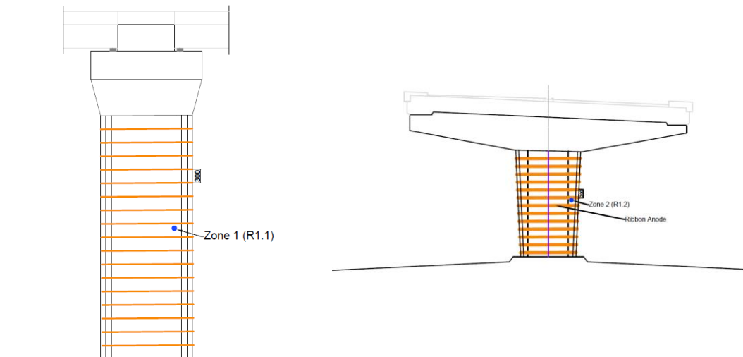
(a) North Elevation Column: Zone 1 (North and South combine)
