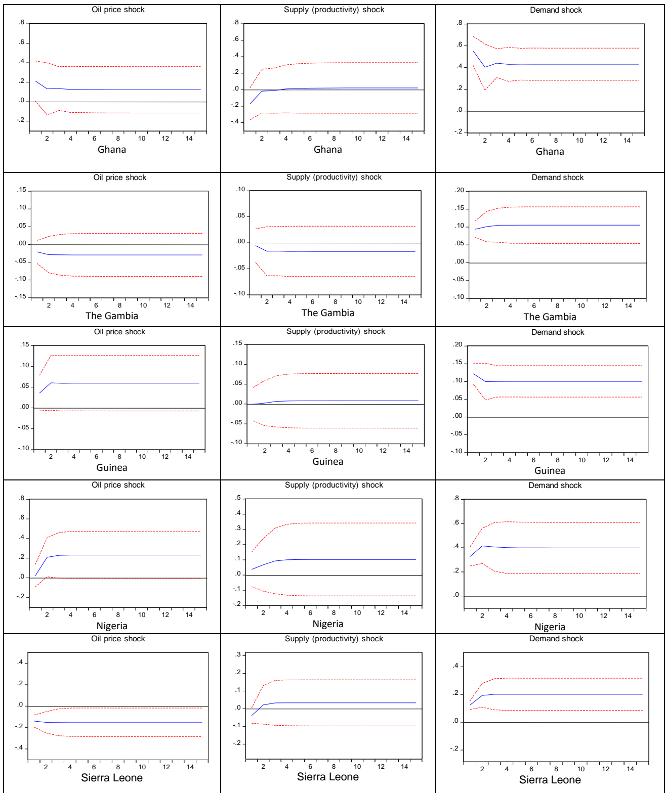
Figure 3: Cumulated impulse responses of real effective exchange rates to one standard deviation structural innovations.
