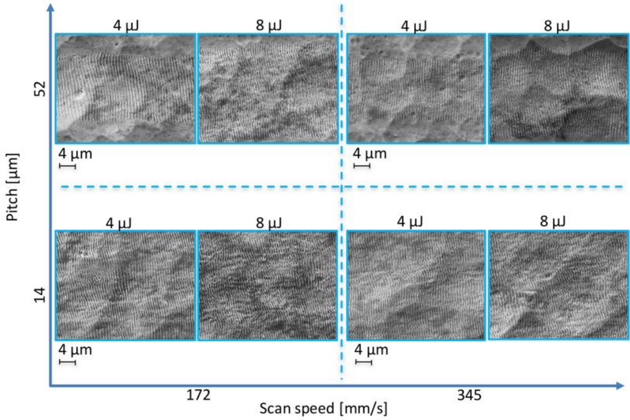
Figure 4. SEM images of the surfaces obtained as a function of process parameters with ps-pulsed fiber laser at 1064 nm.
