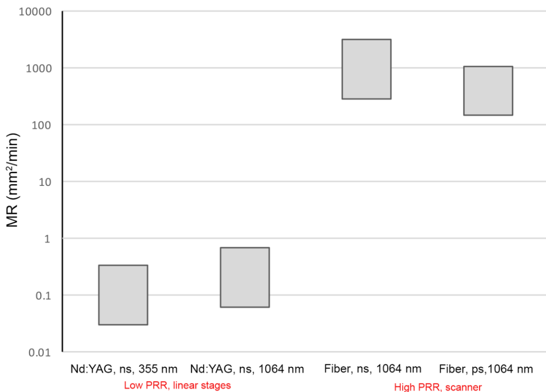
Figure 11. Machining rates of the tested configurations.
