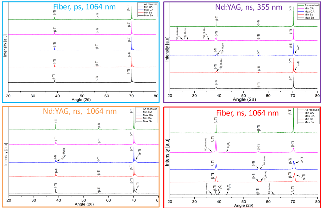
Figure 10. XRD analysis of the representative conditions obtained with each laser source.
