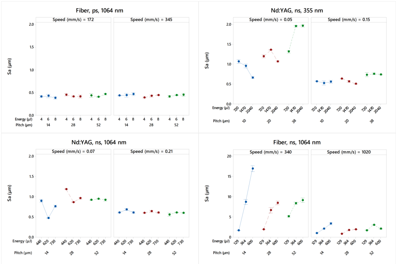
Figure 8. Average surface roughness ( S_a ) obtained as a function of process parameters and laser configurations. Note the different scale for the ns-pulsed fiber laser with 1064 nm wavelength, which is larger for readability.
